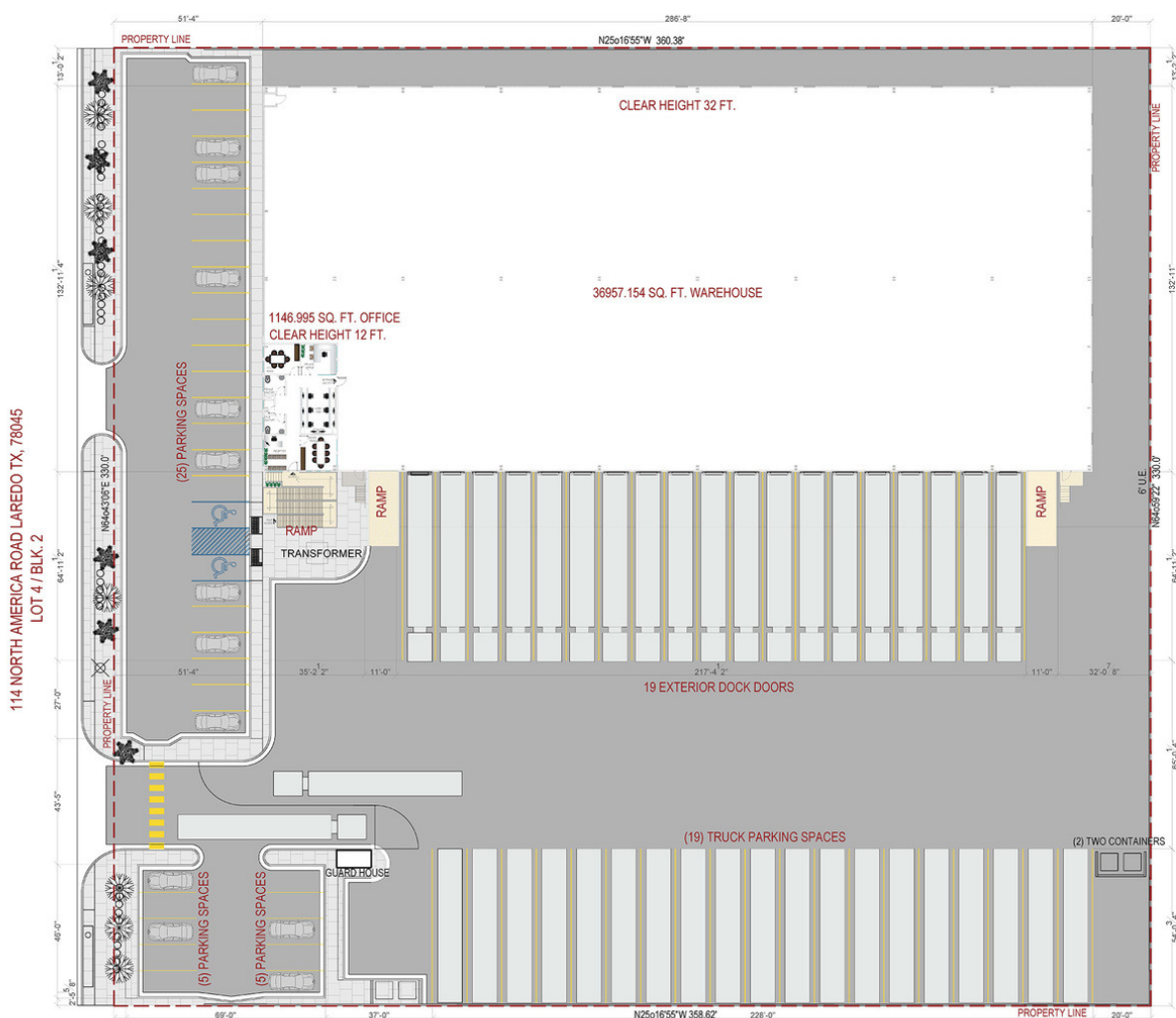
SITE PLAN
