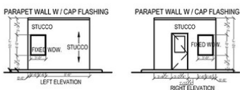
ELEVATIONS - GUARD HOUSE
