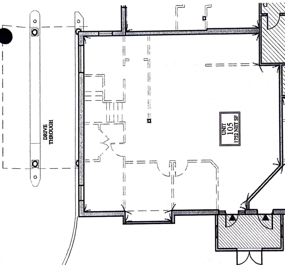
UNIT 105 FIRST FLOOR
