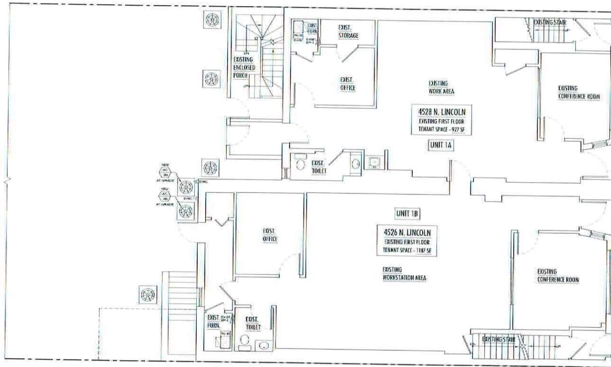
A EXISTING FIRST FLOOR PLAN SCALE: 1/4" = 1'-0" FOR REFERENCE ONLY - NO PERMITS
