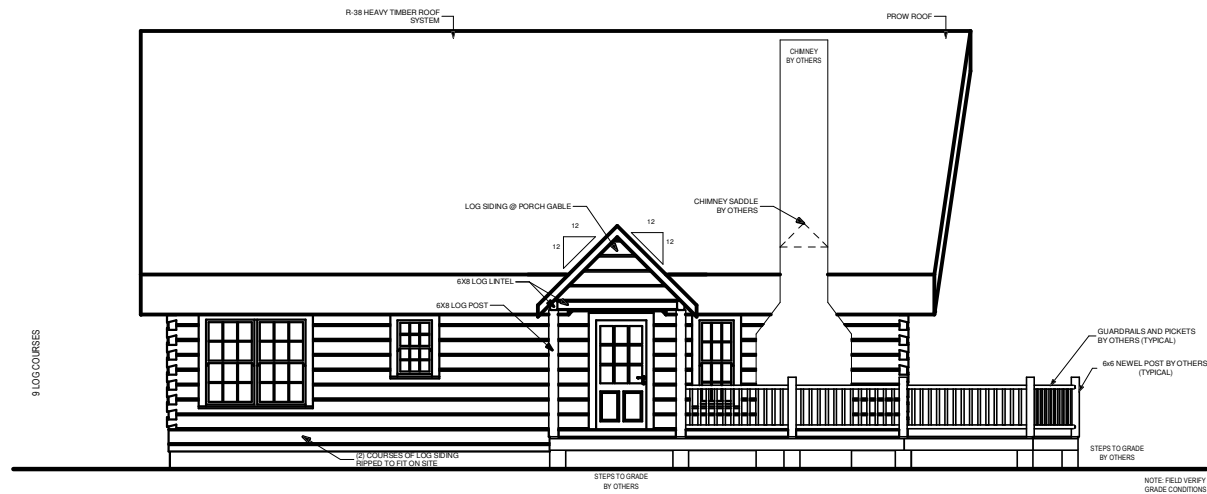
LEFT ELEVATION
