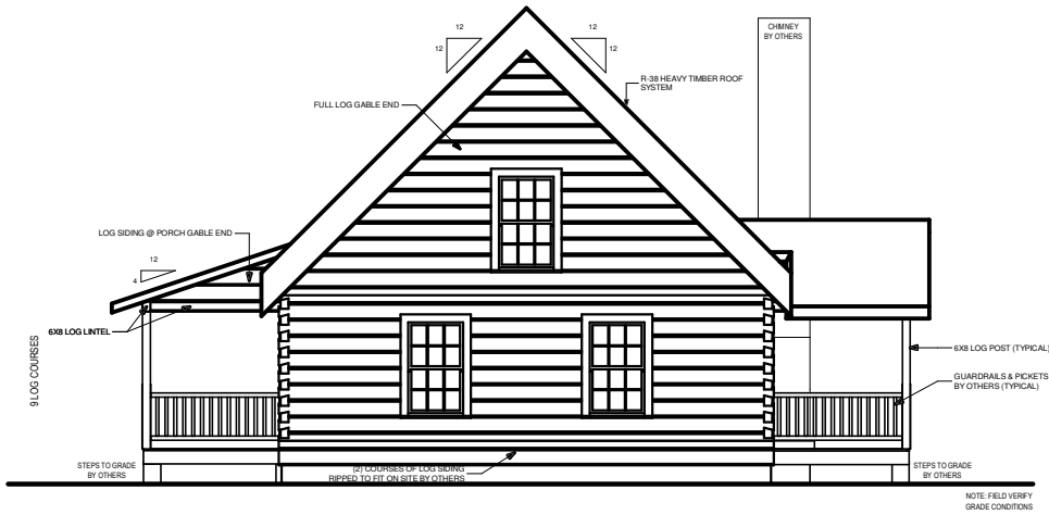
REAR ELEVATION
