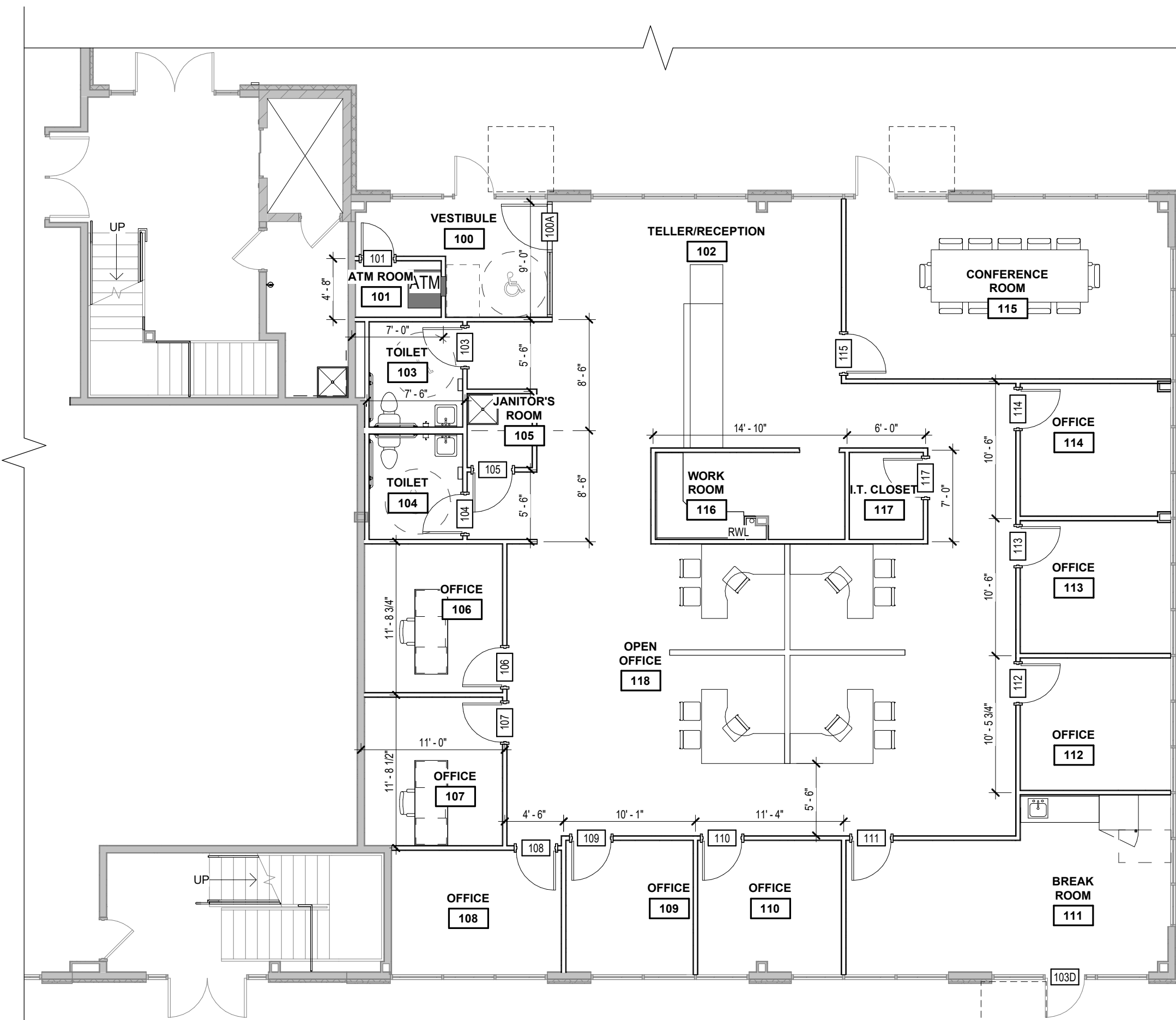
1 FIRST LEVEL FLOOR PLAN 1/8" = 1'-0"
