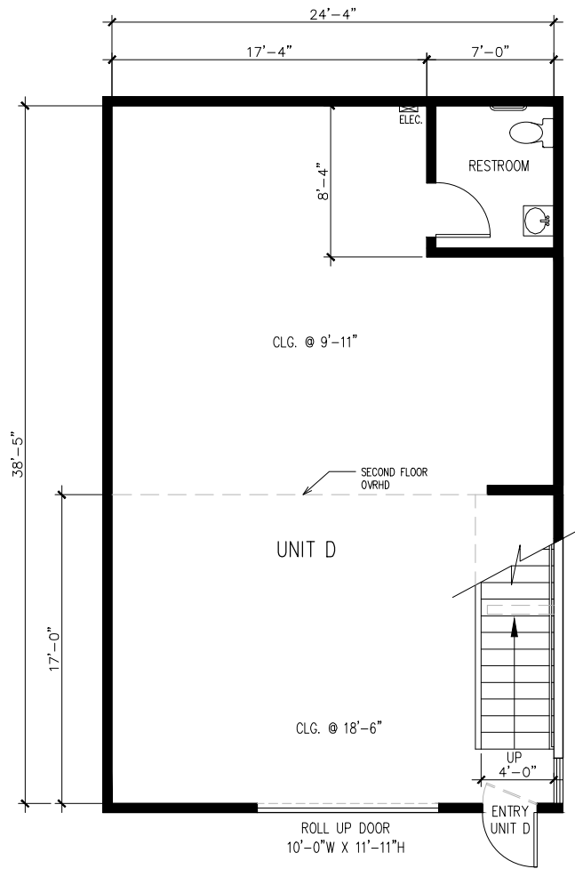
FIRST FLOOR PLAN - UNIT D (935 SQ. FT. +/-) NTS
