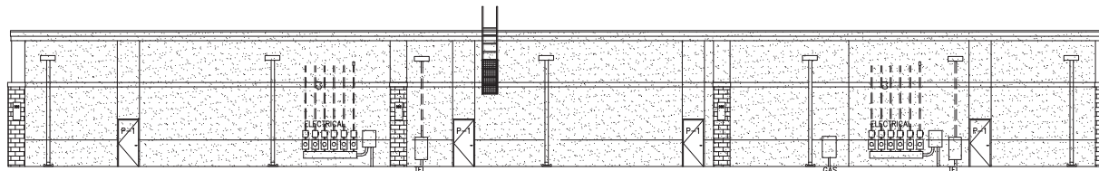
3 EXTERIOR ELEVATION 1/8" WEST - BUILDING 'B'
