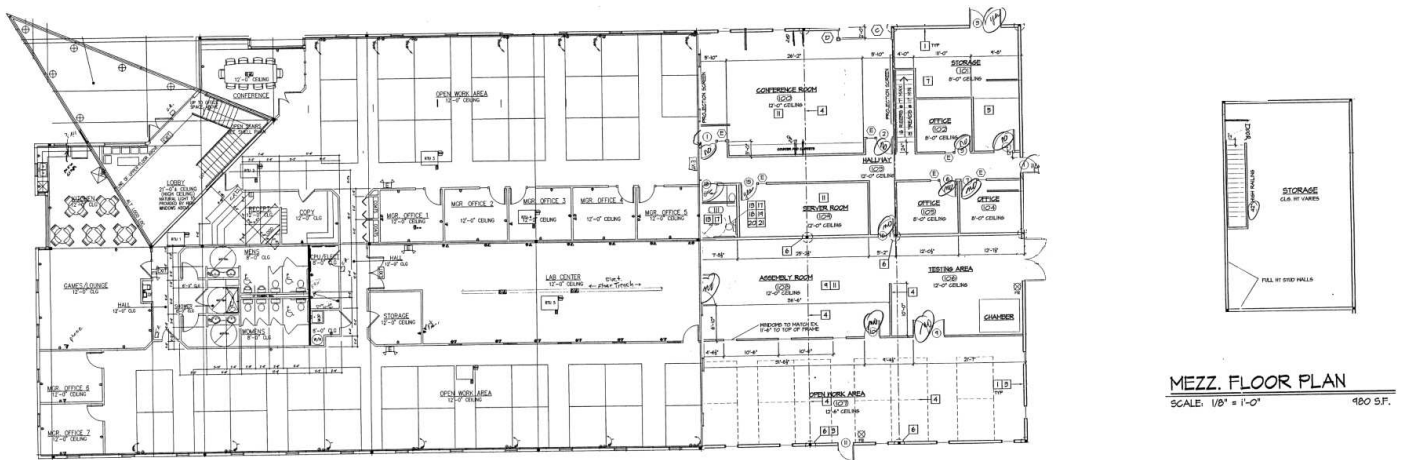
1 story FLOOR PLAN NEW ADDITION 5000 S.F. SCALE: 1/8" = 1'-0"
