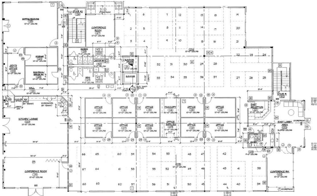
First Floor of 2-Story Addition
