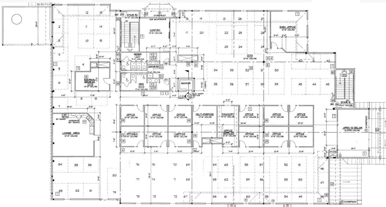
Second Floor of 2-Story Addition
