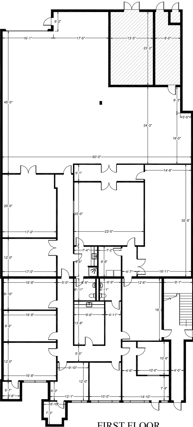
FIRST FLOOR
