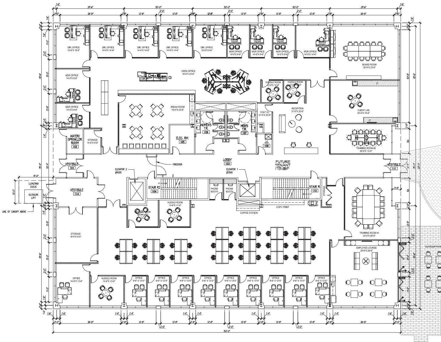
1st Floor-Space Plan
