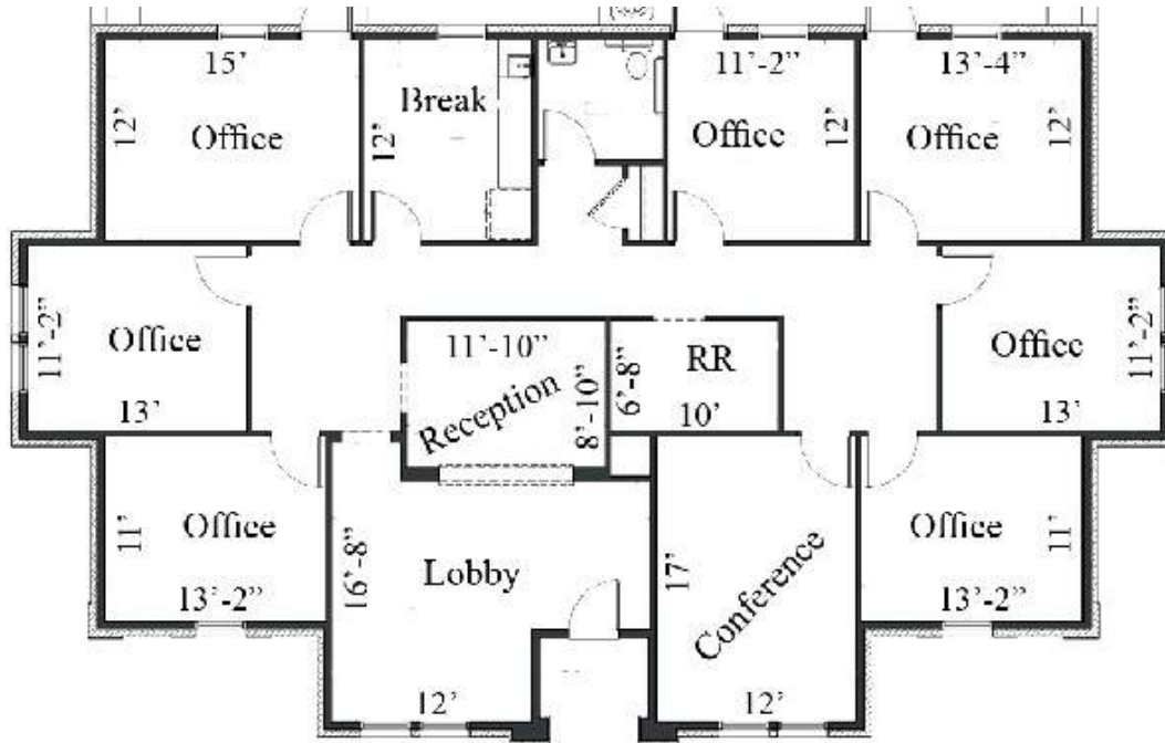
Preliminary floor plan subject to modification
