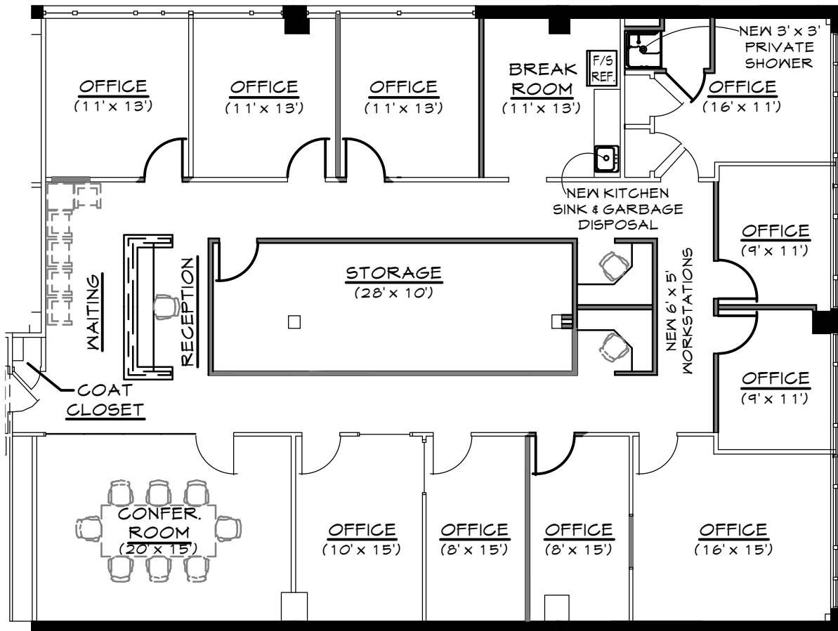
2ND FLOOR KEY PLAN
