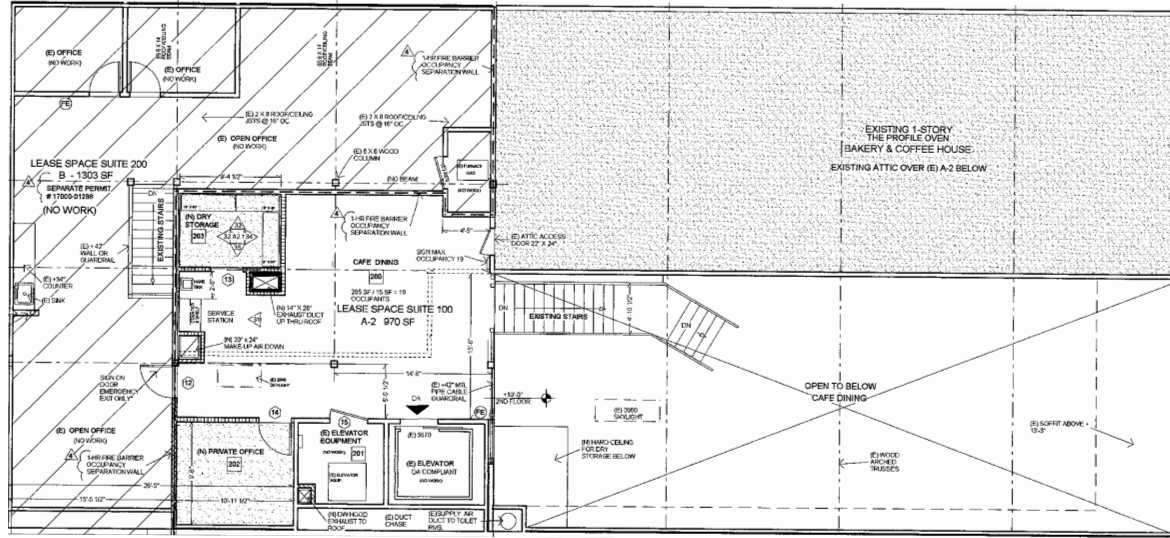
MEZZANINE LEVEL
