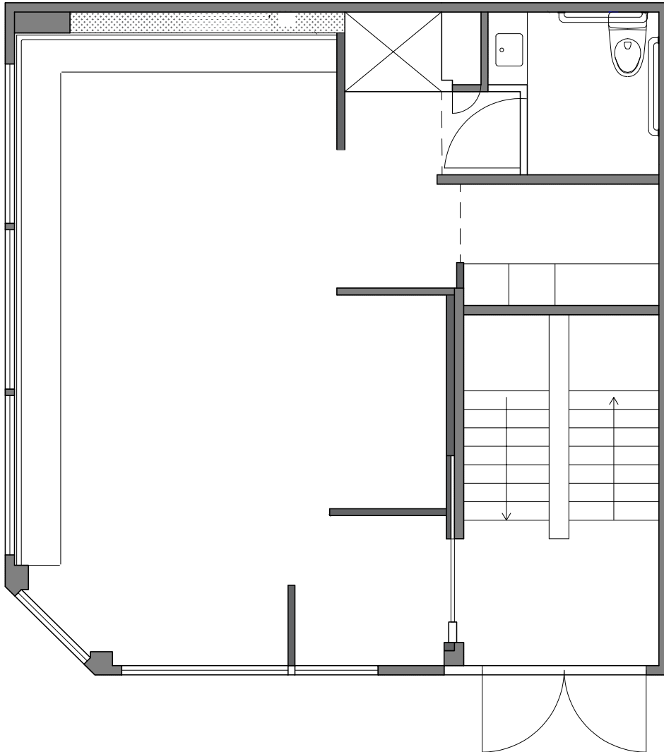
FLOOR PLANS: GROUND FLOOR - 700 SF
