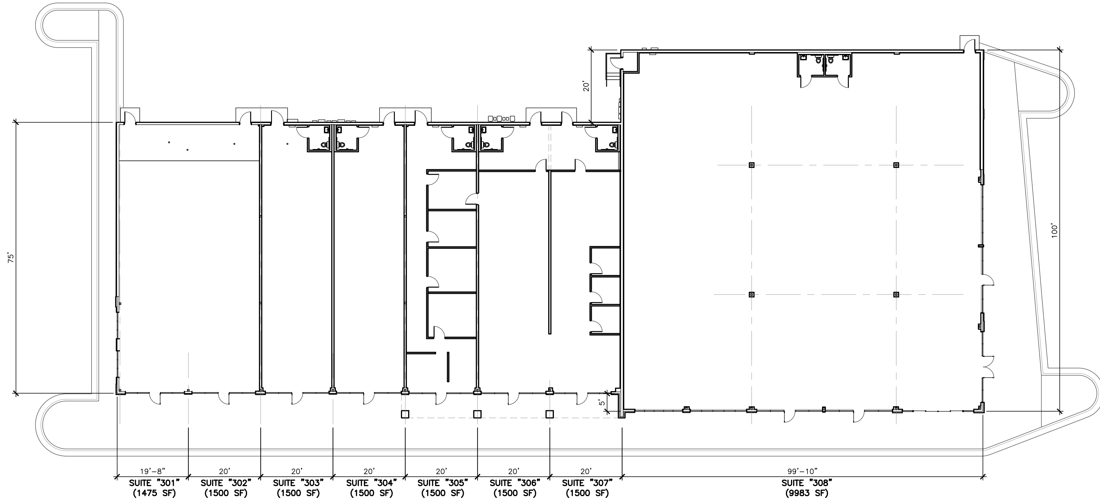
OVERALL FLOOR PLAN - BUILDING "C" 1/16" = 1'-0"
