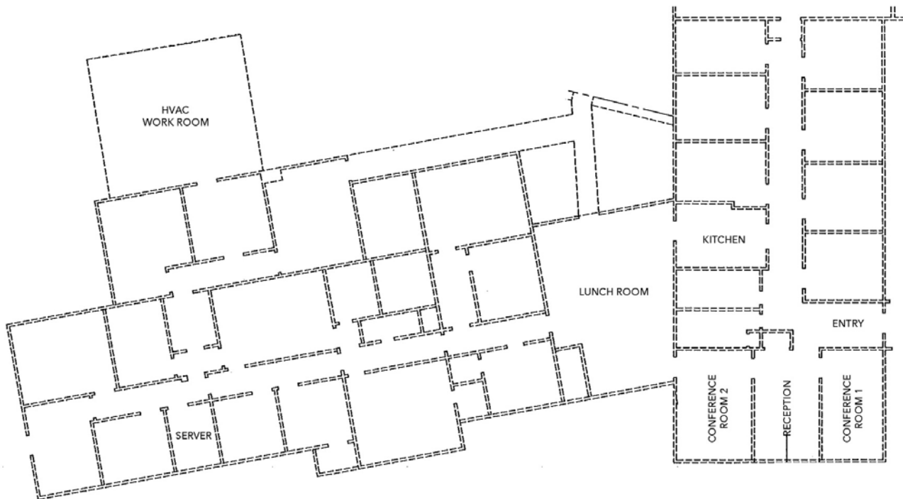
1221 OFFICE FLOOR PLAN
