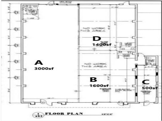
Floor Plan 2155 Building -6550sf
