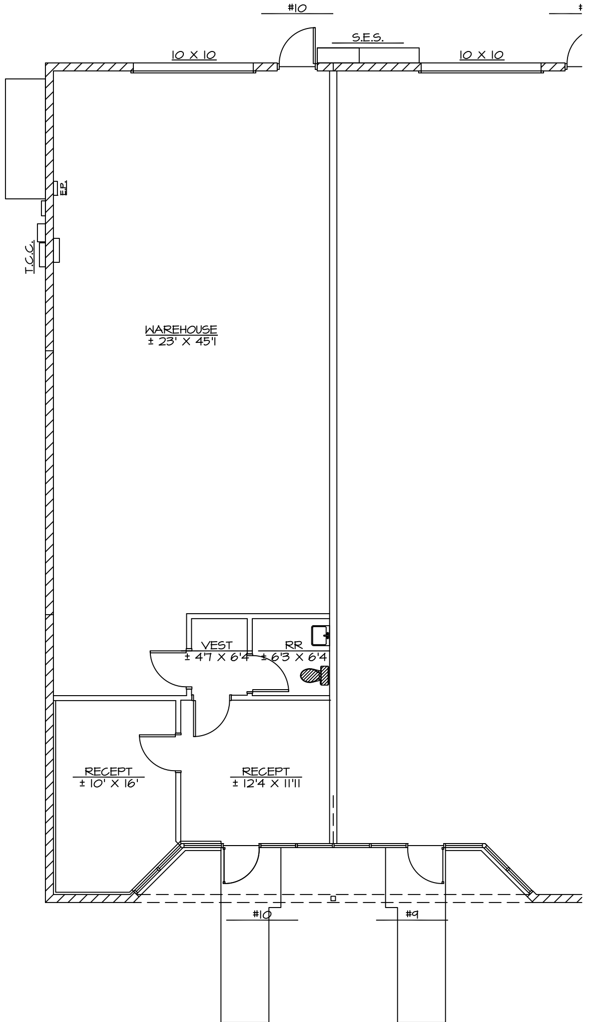
FLOOR PLAN
