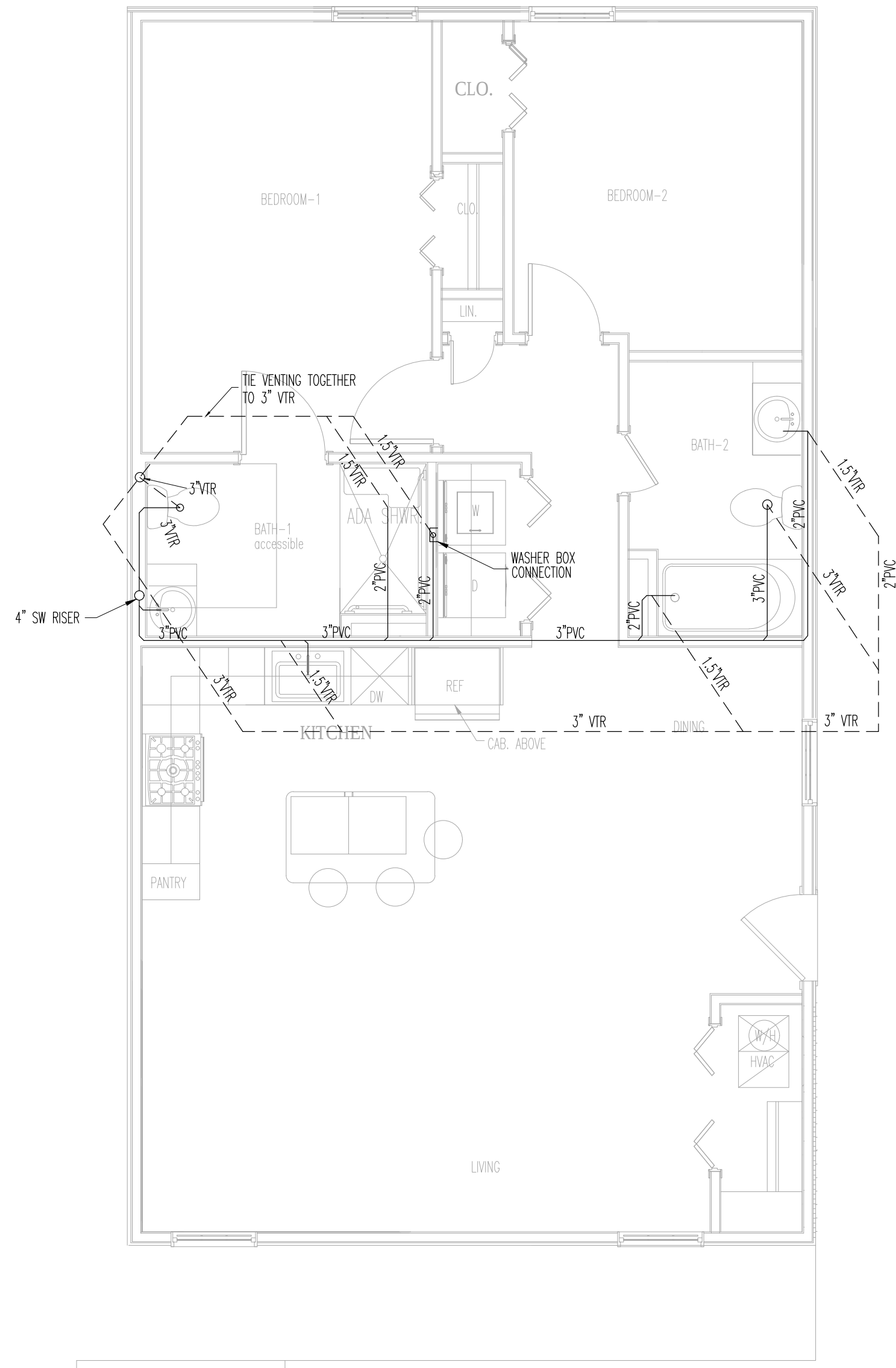
1 SANITARY WASTE PLAN SCALE: 1/4"=1'-0"
