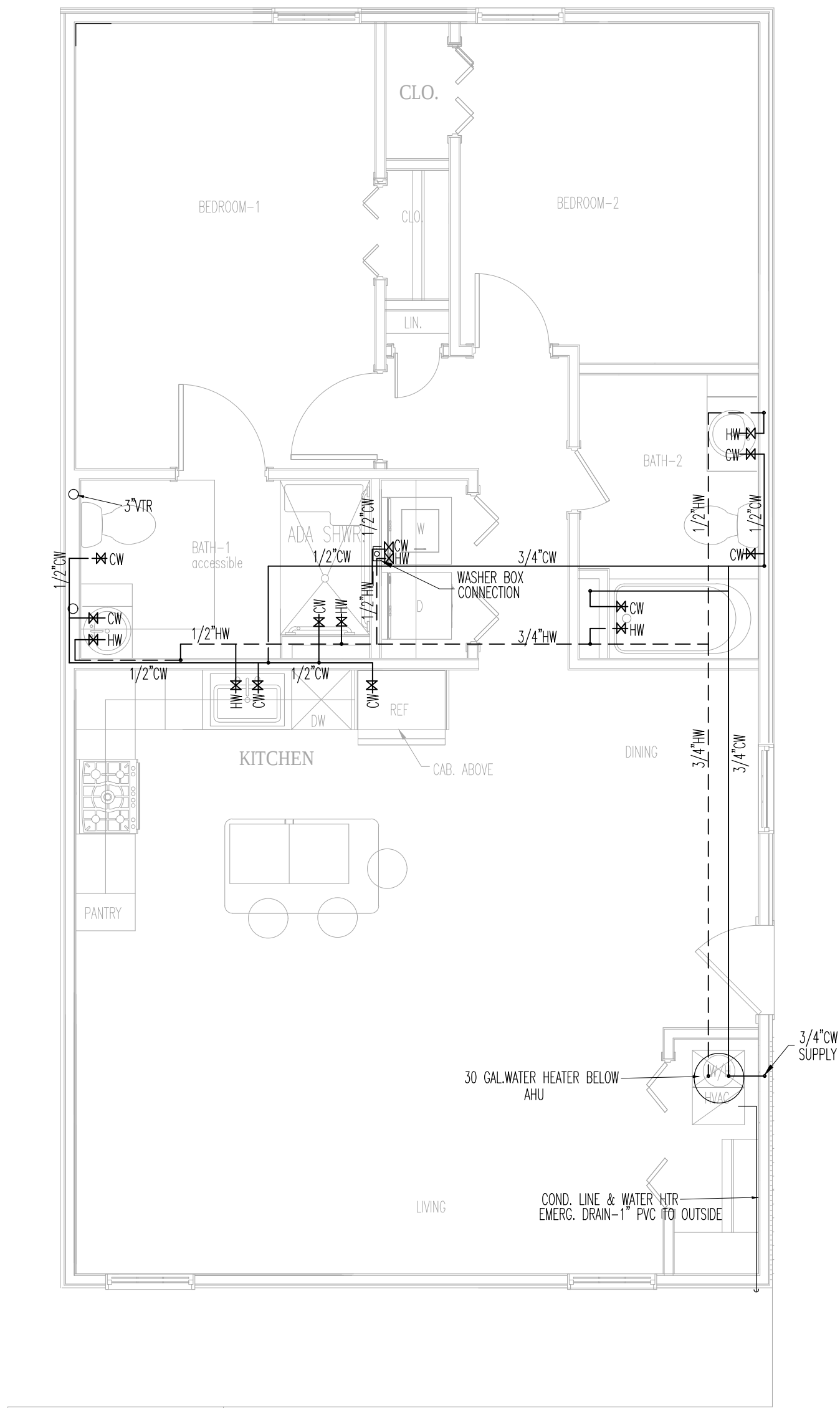
2 WATER SUPPLY PLAN SCALE: 1/4"=1'-0"
