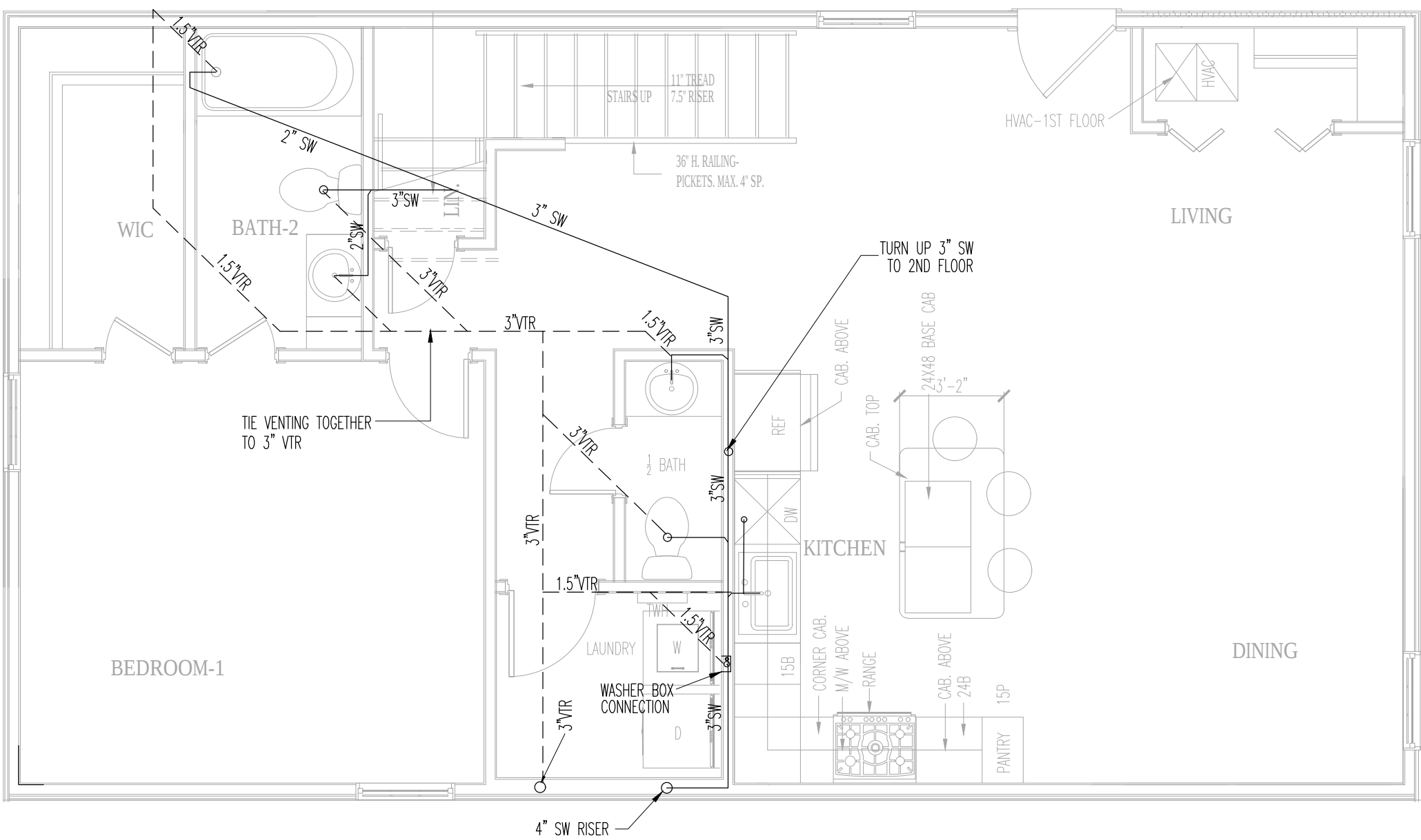
FIRST FLOOR
