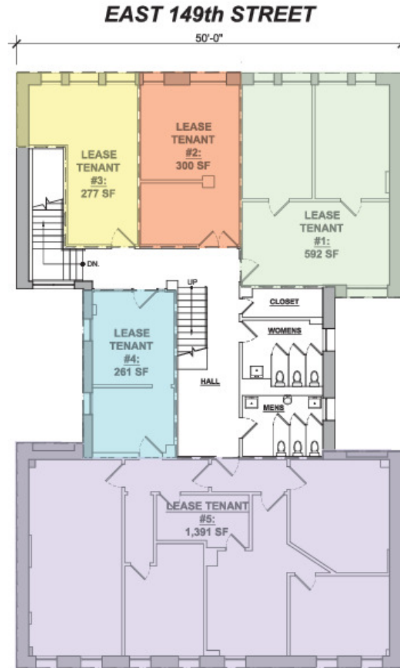
SECOND FLOOR
