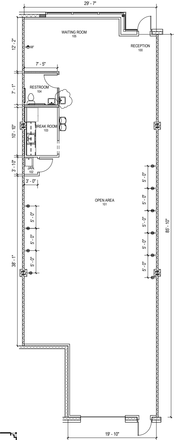
FLOOR PLAN
