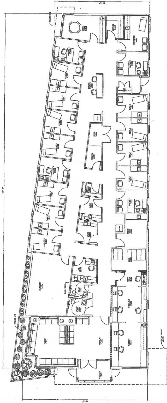
NORTH FIRST FLOOR PLAN SCALE 3/16" = 1'-0"
