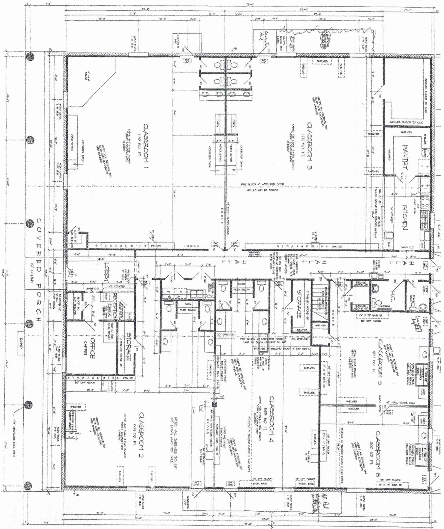
FLOOR PLAN
