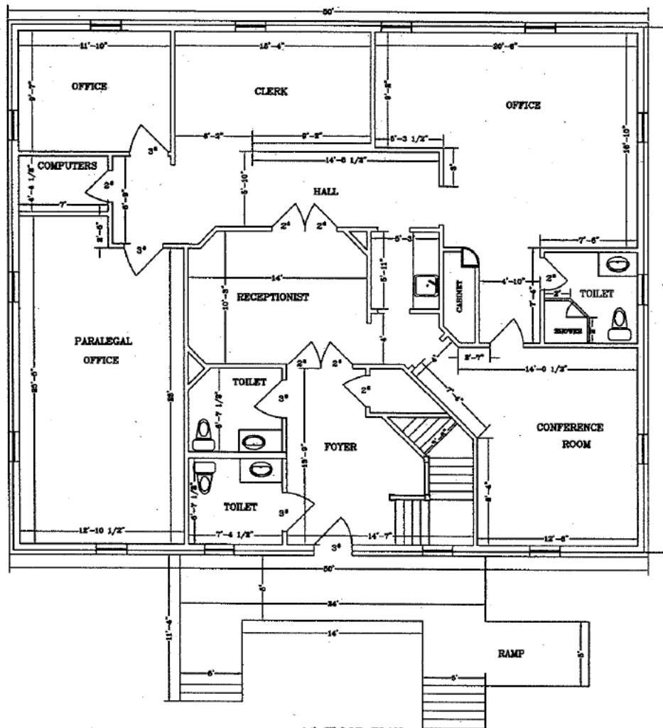
1 st FLOOR PLAN SCALE 1/4" = 1'-0"
