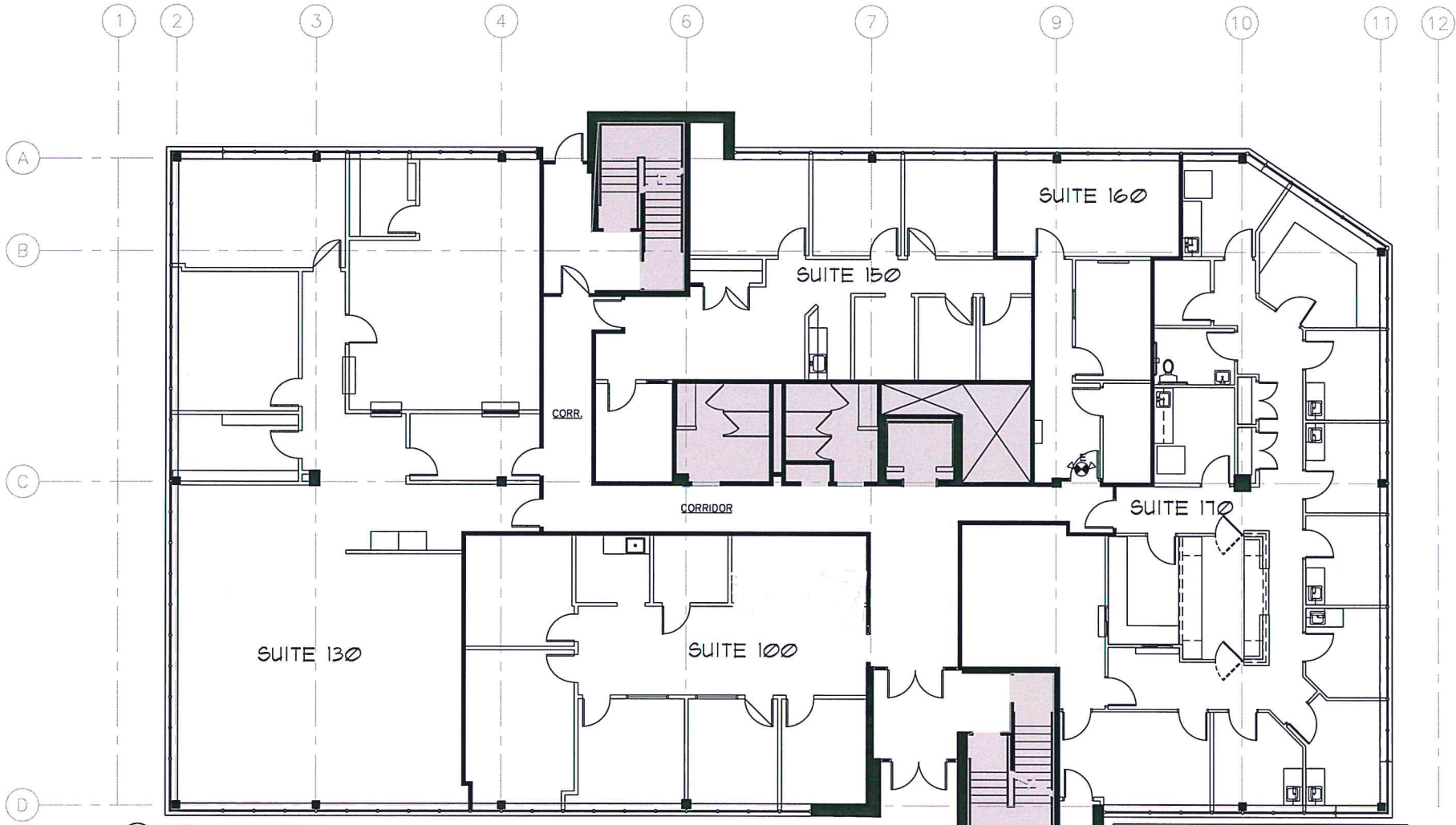
1 EXISTING FIRST FLOOR PLAN FP-1.1 SCALE: 1/4" = 1'-0"
