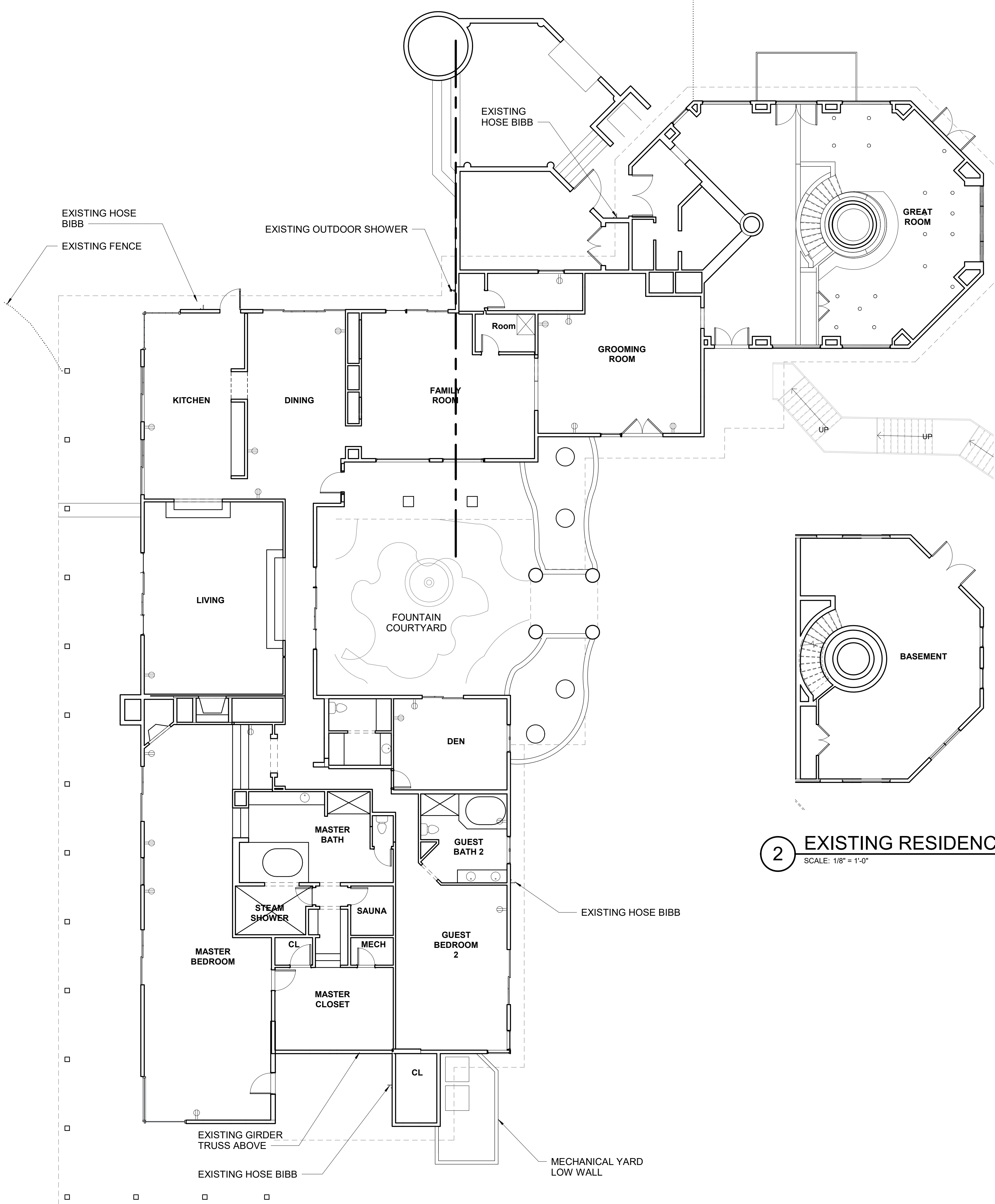
1 EXISTING RESIDENCE - LEVEL 1 SCALE: 1/8" = 1'-0"
