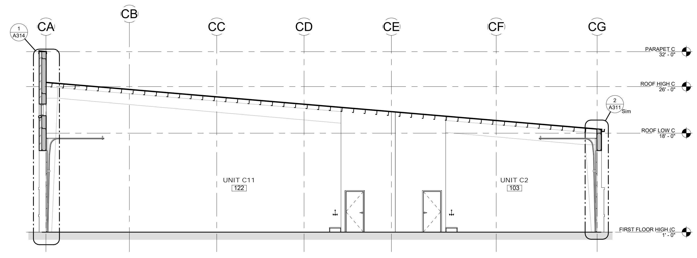
2 BUILDING SECTION 1/8" = 1'-0"
