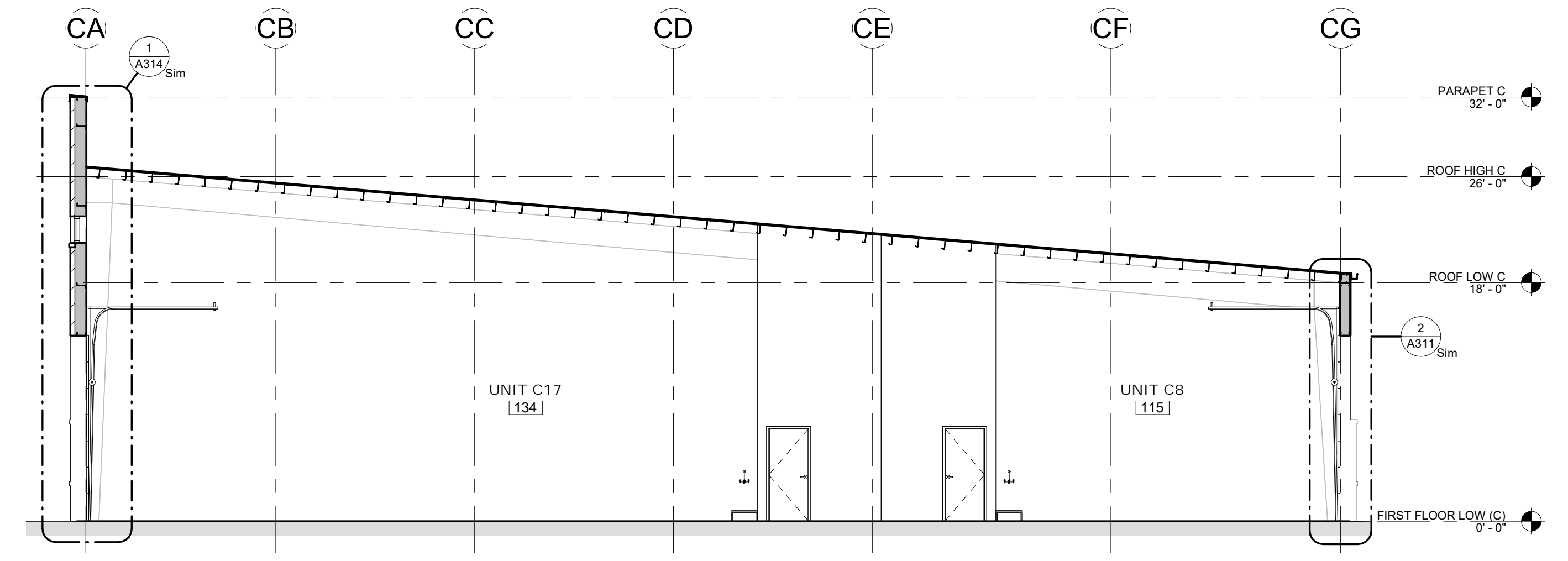
4 BUILDING SECTION 1/8" = 1'-0"
