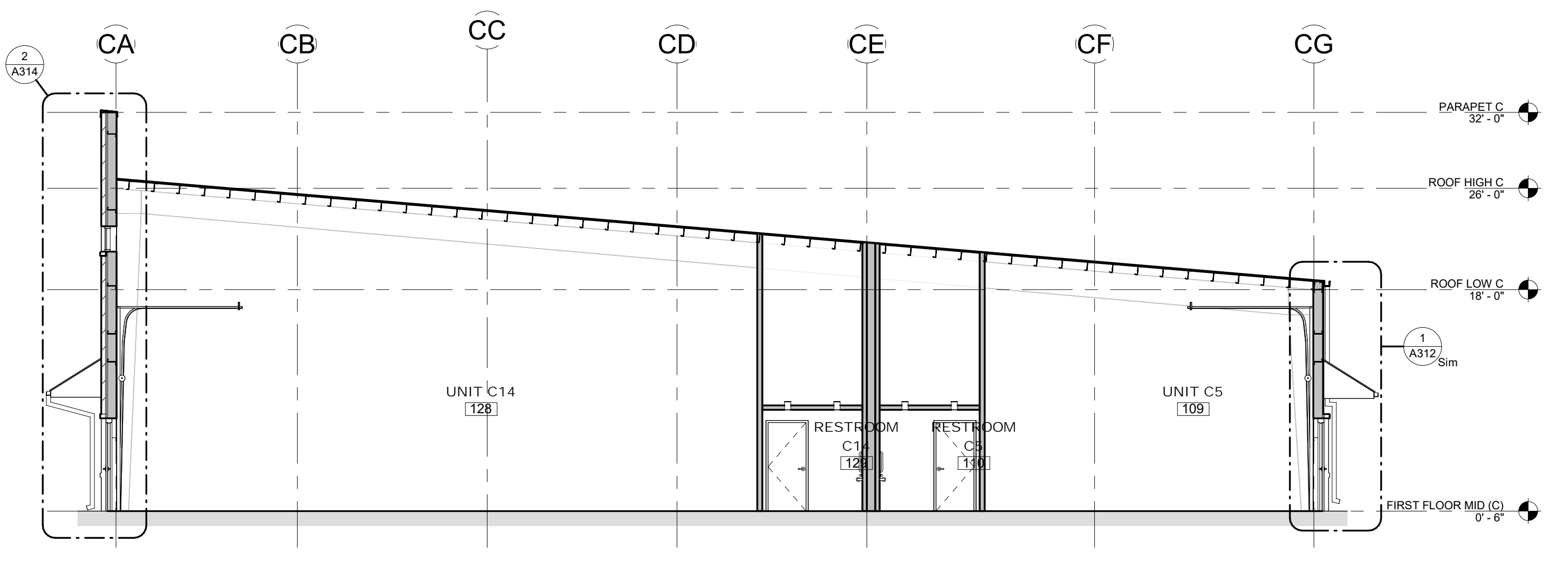
3 BUILDING SECTION 1/8" = 1'-0"
