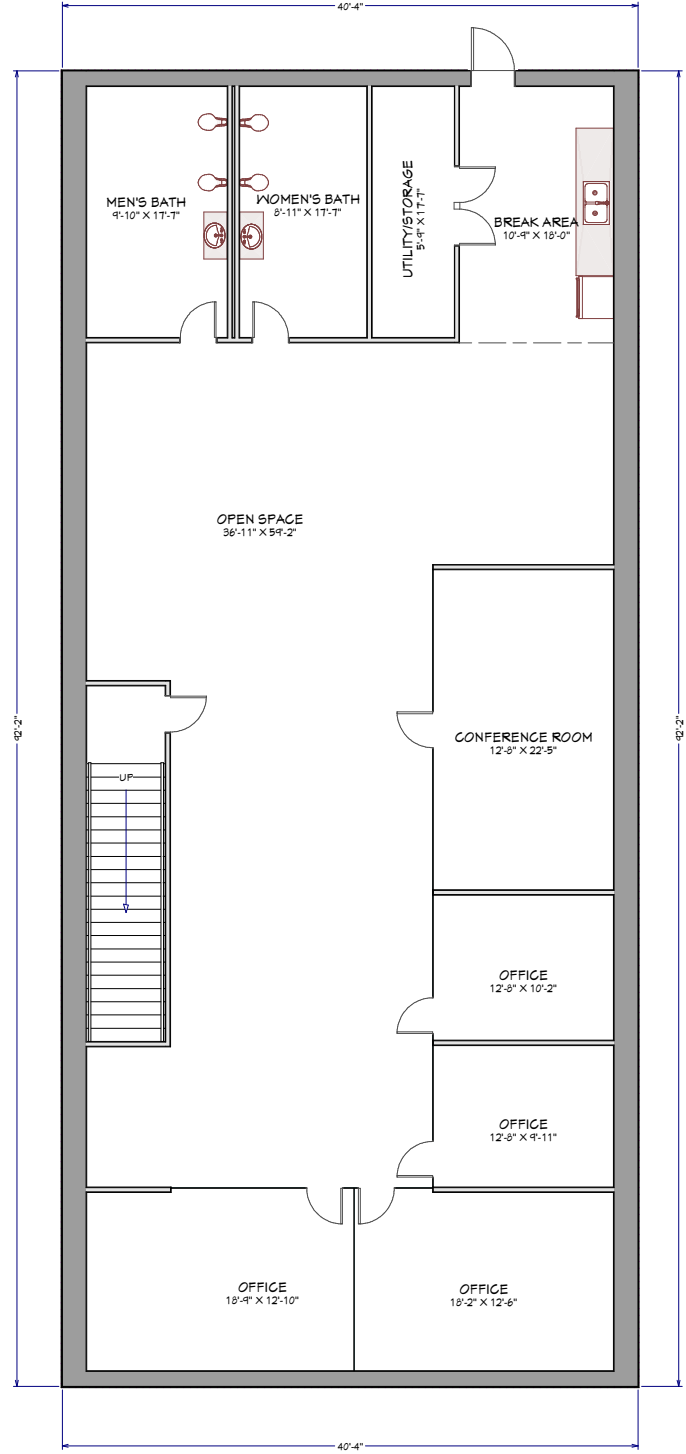
SECOND FLOOR 3117 SQ FT
