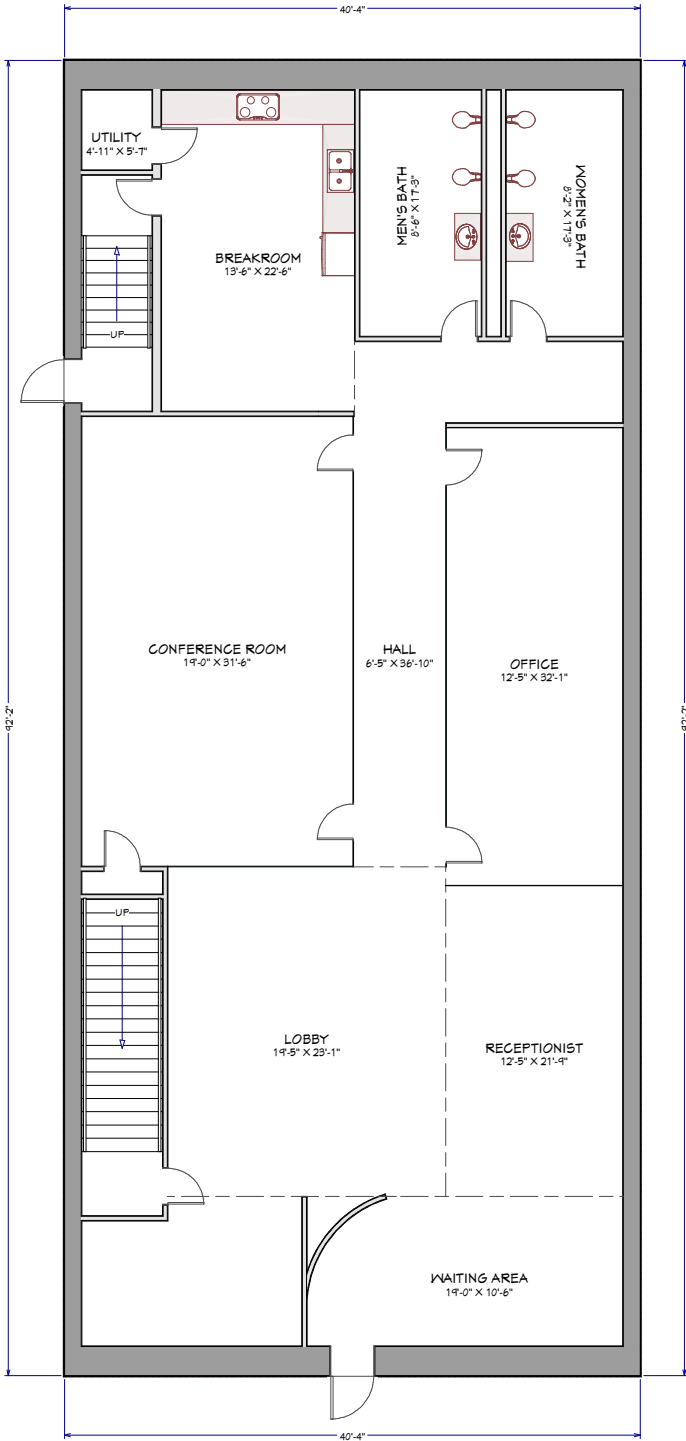
FIRST FLOOR 3117 SQ FT
