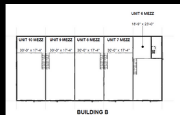
MEZZANINE LAYOUT
