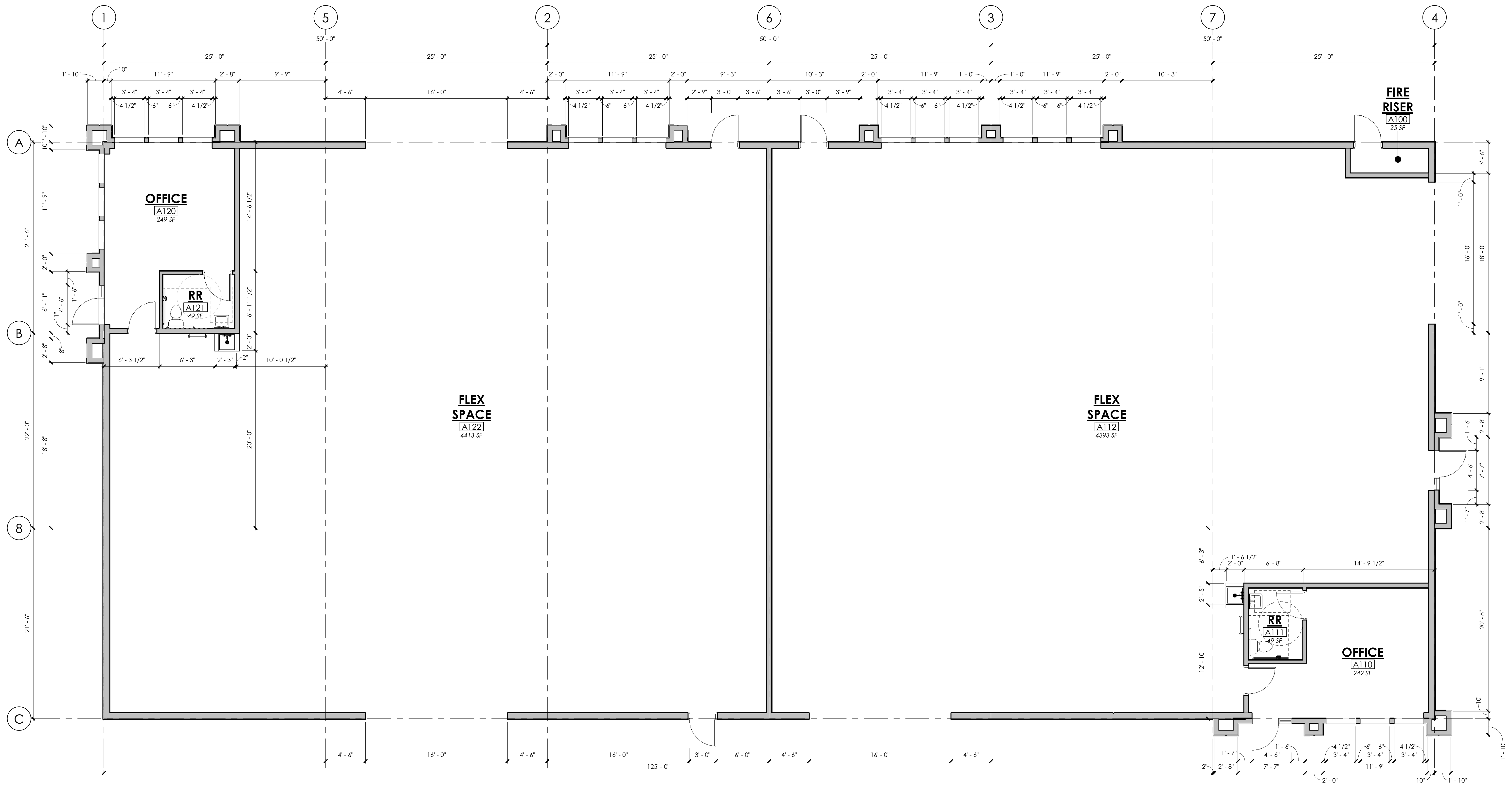
1 FLOOR PLAN 3/16" = 1'-0"
