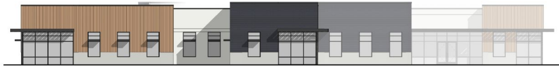
21 A201 SOUTH WEST ELEVATION 1/8" = 1'-0"
