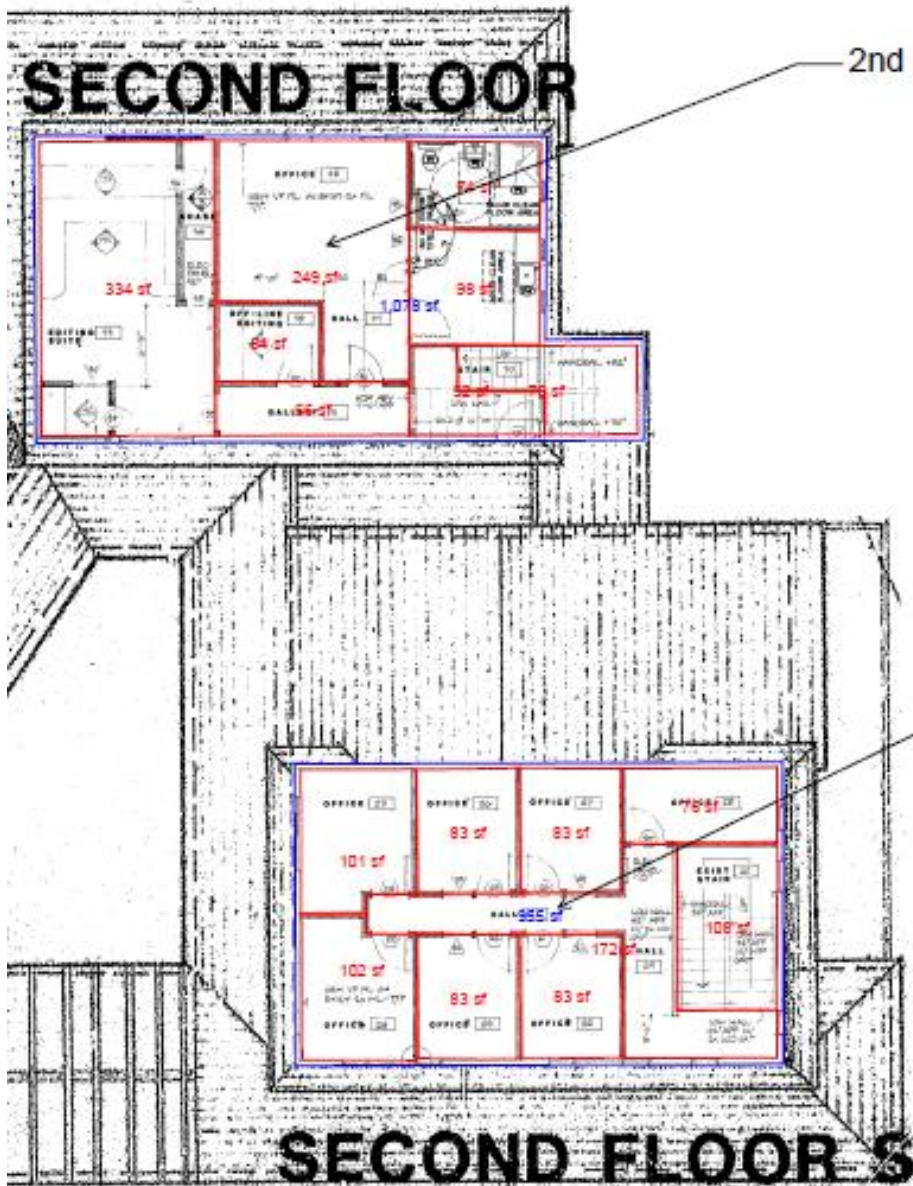
2nd Floor - Section D (Office)
