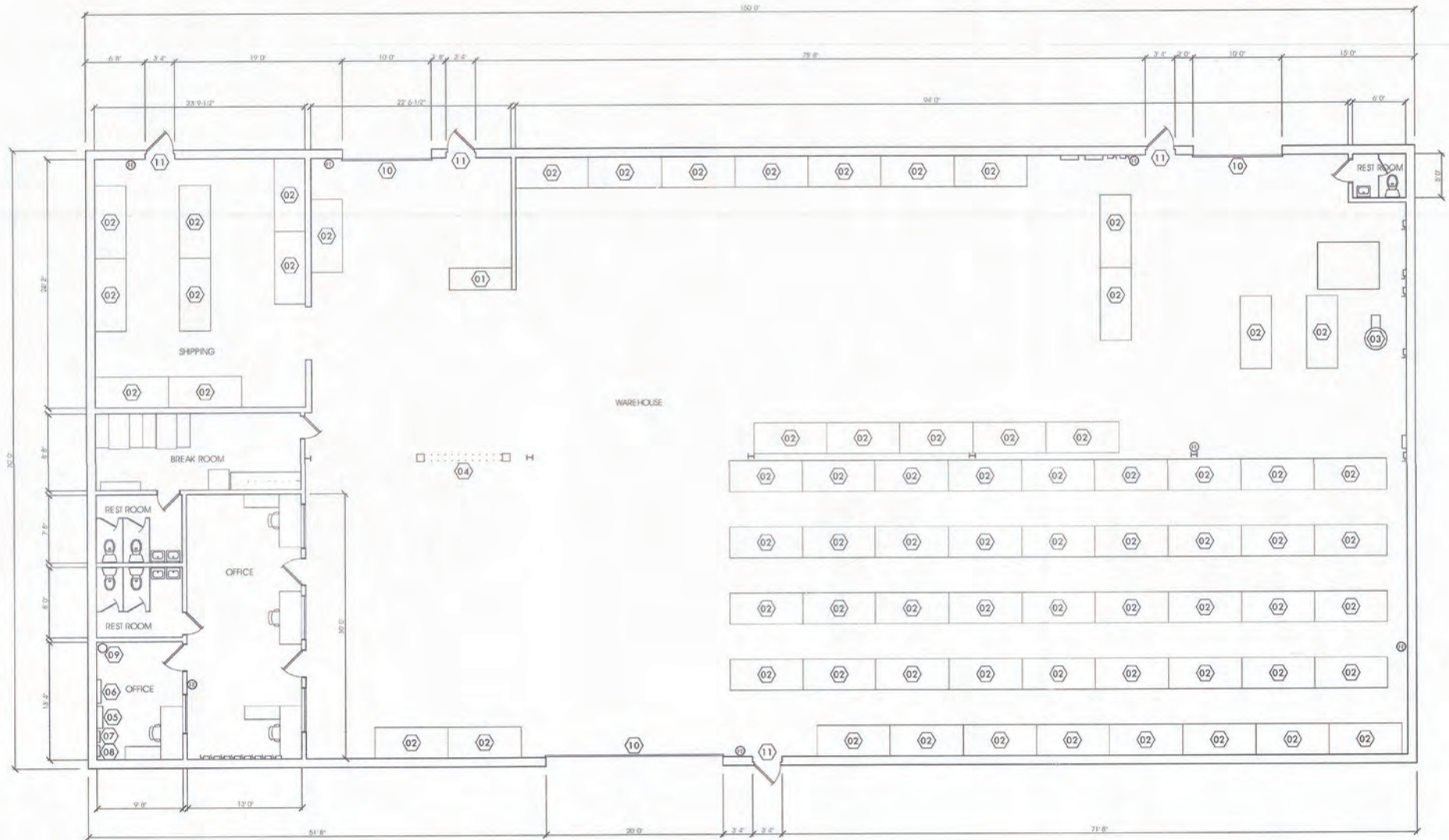
Ground Floor Plan 1/8" = 1'-0"
