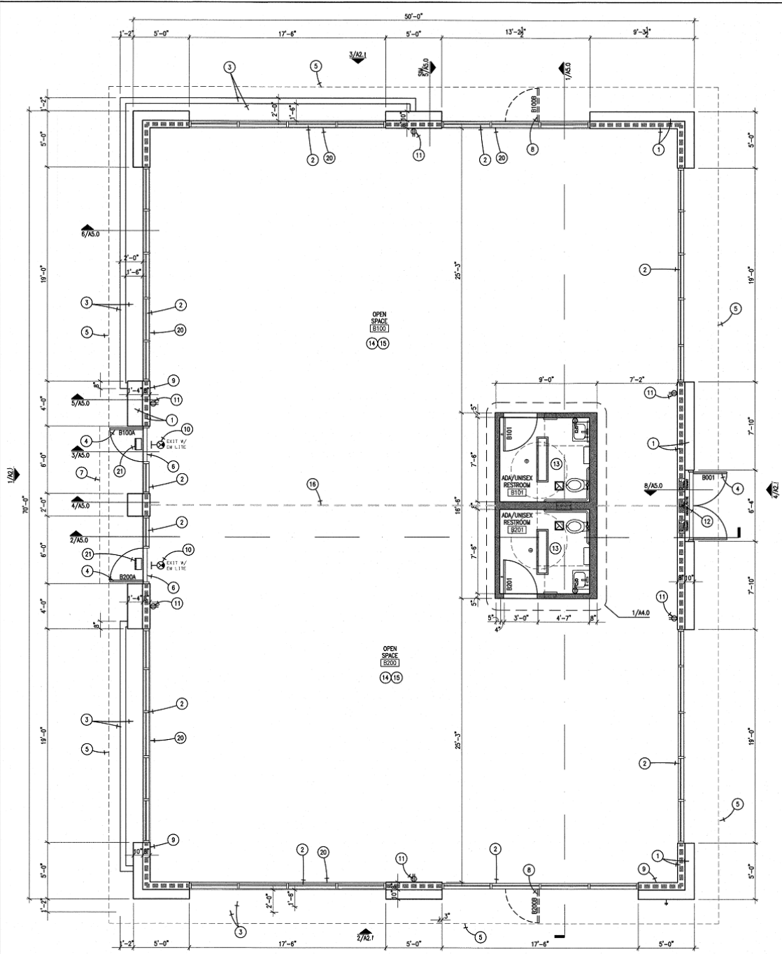
FLOOR PLAN - BLDG 'B' SCALE: 1/4"=1'-0"
