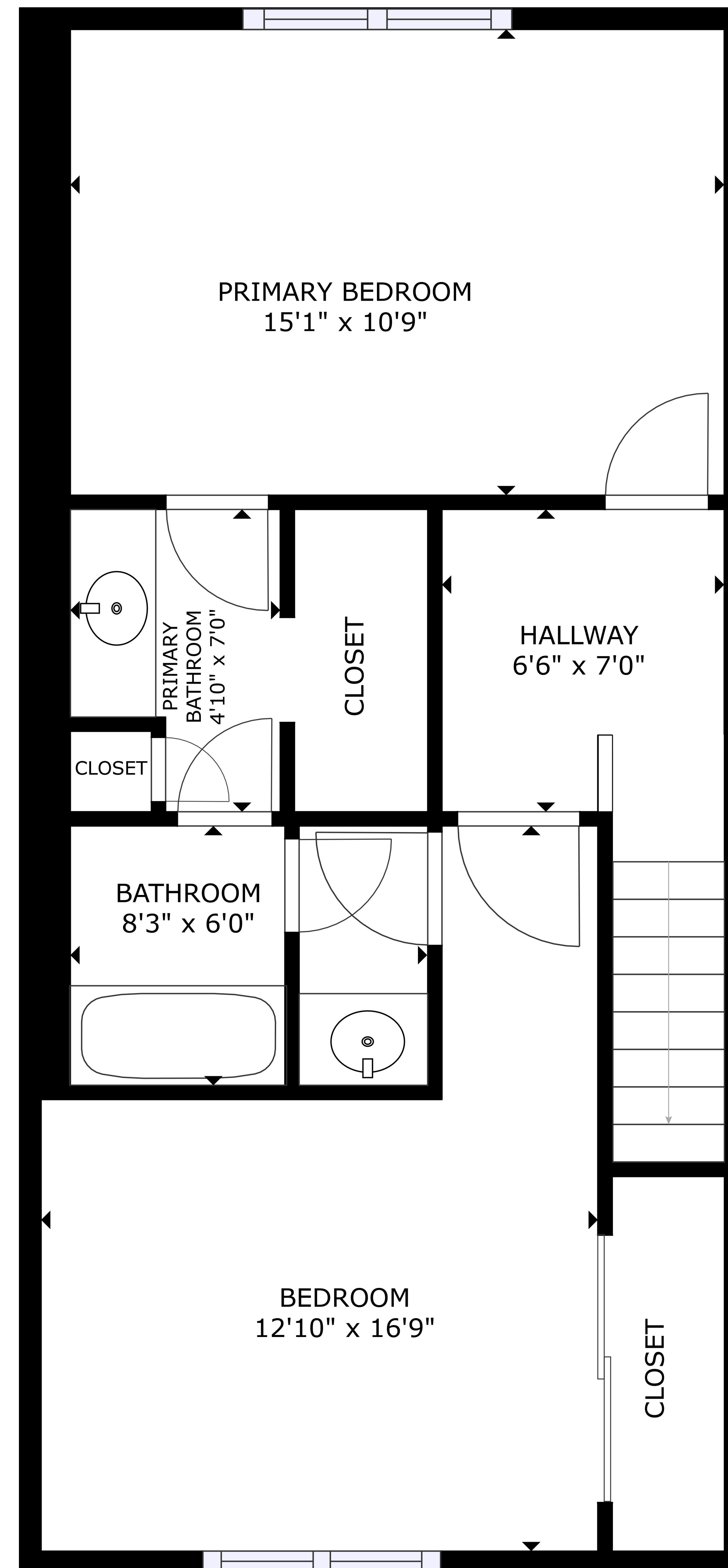
FLOOR 2
