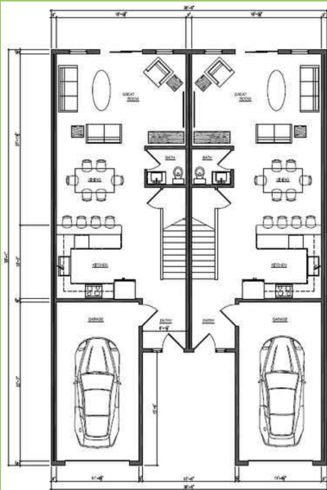
FIRST FLOOR PLAN UNIT 'A'
