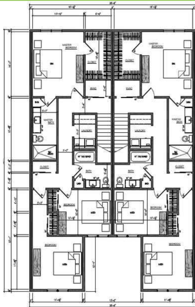
SECOND FLOOR PLAN UNIT 'A'
