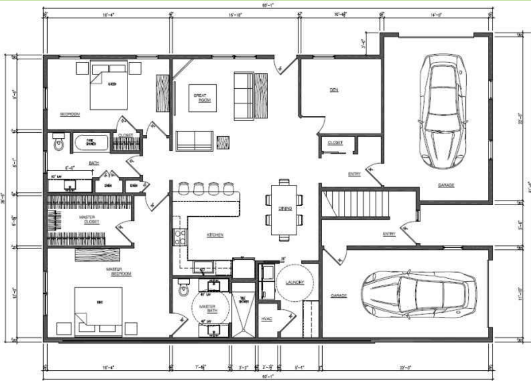
FIRST FLOOR PLAN UNIT 'C'
