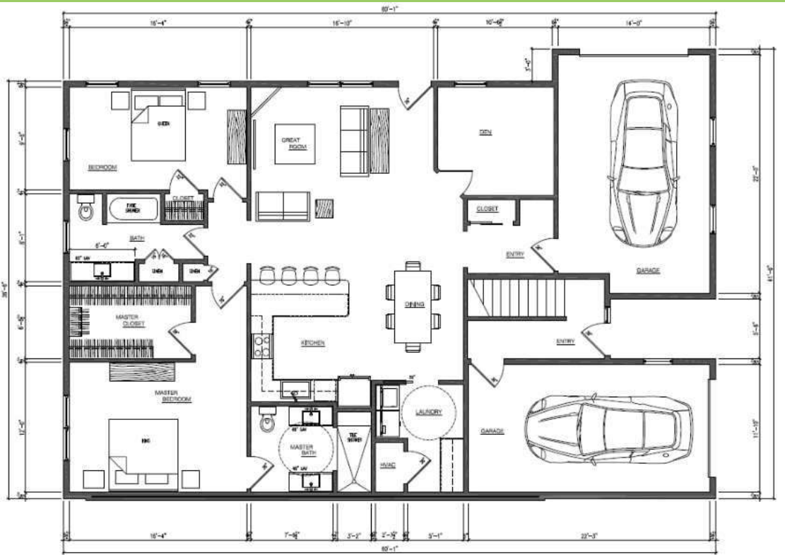
FIRST FLOOR PLAN UNIT 'C'
