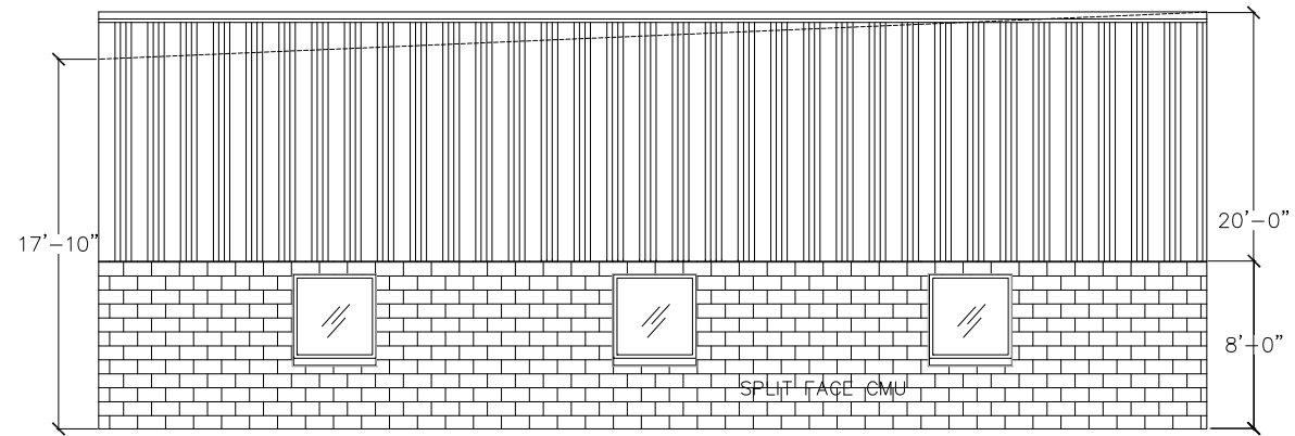
FRONT ELEVATION FACING CHURCH STREET
