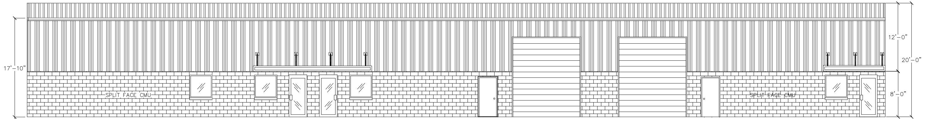
FRONT ELEVATION FACING GOLDEN SPIKE LANE
