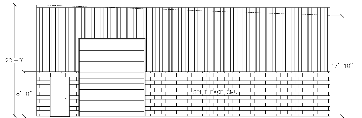
BACK ELEVATION FACING CABOOSE PLACE
