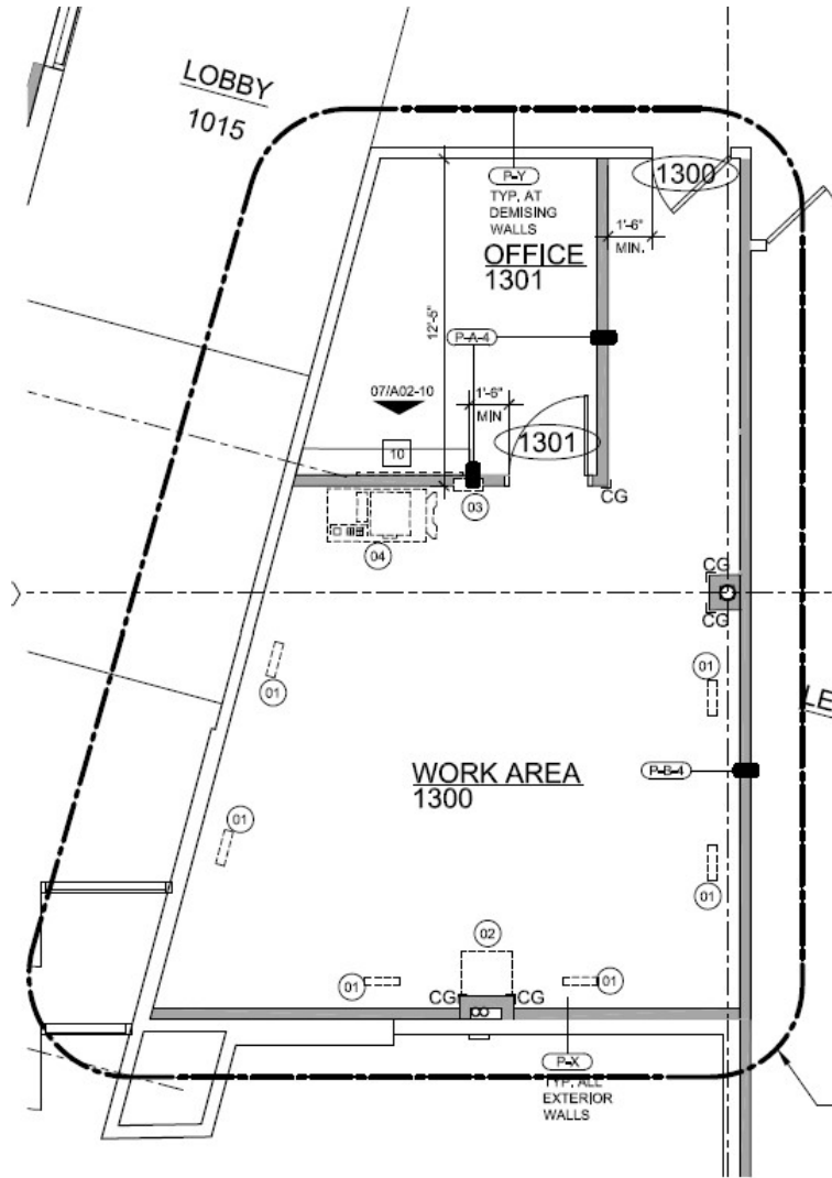
01 FLOOR PLAN SCALE: 1/4" = 1'-0"
