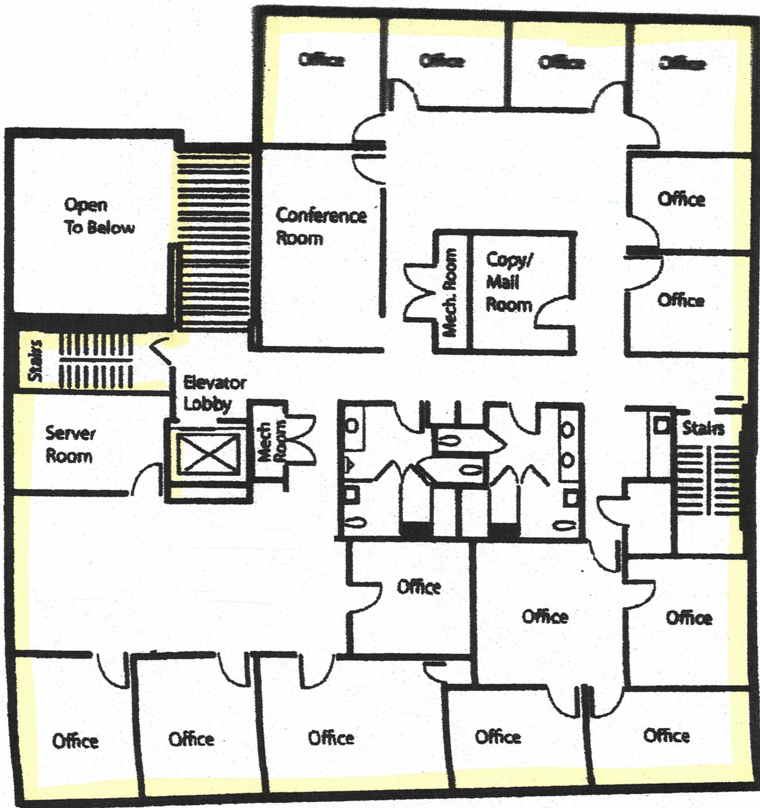
FLOOR PLAN | Suite B - 5,096 SF
