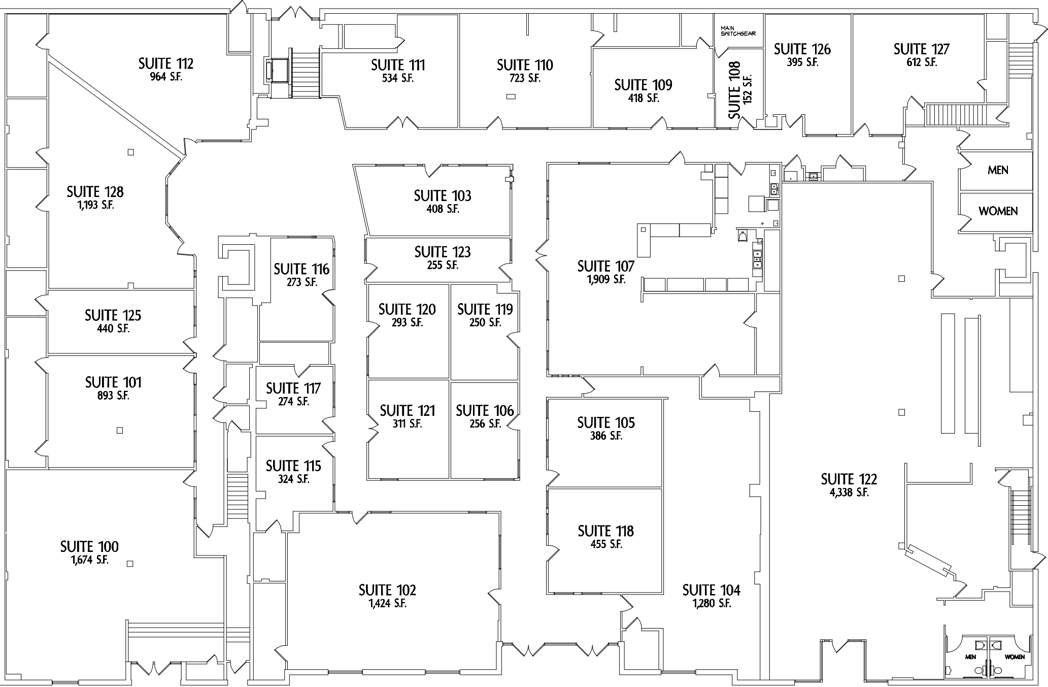
FIRST FLOOR PLAN - 25,485 S.F.
