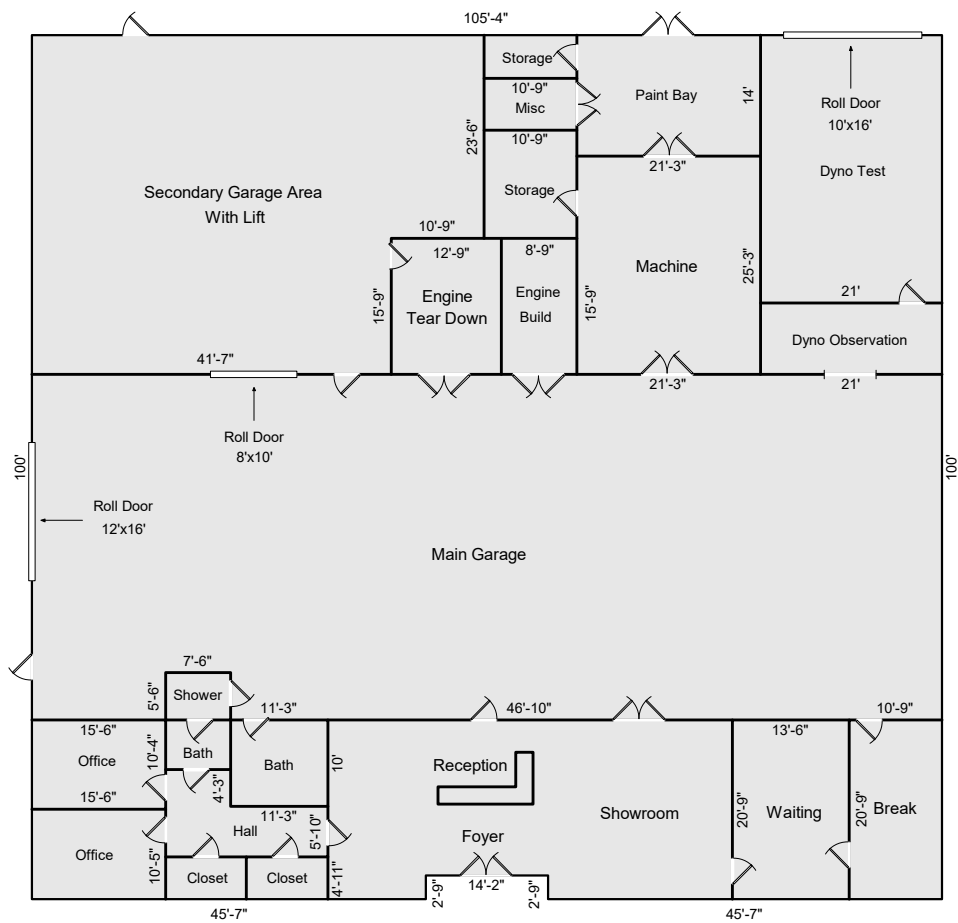
First Floor 10494.4 sf (Approximate Areas) (Dimensions Based On Exterior Measurements)
