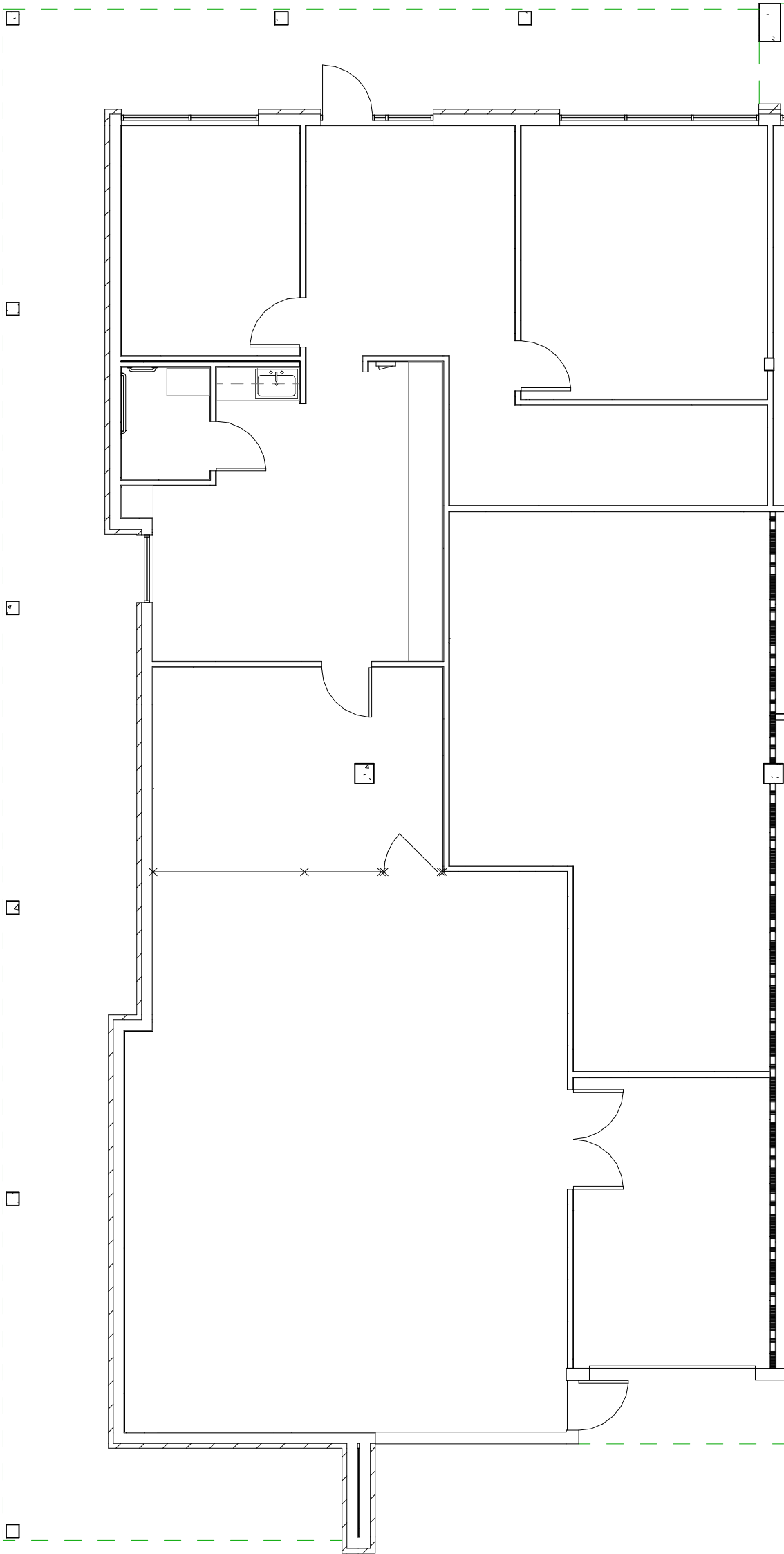
1 Bldg 3000 Suite D - 3,235 SF 1/8" = 1'-0"
