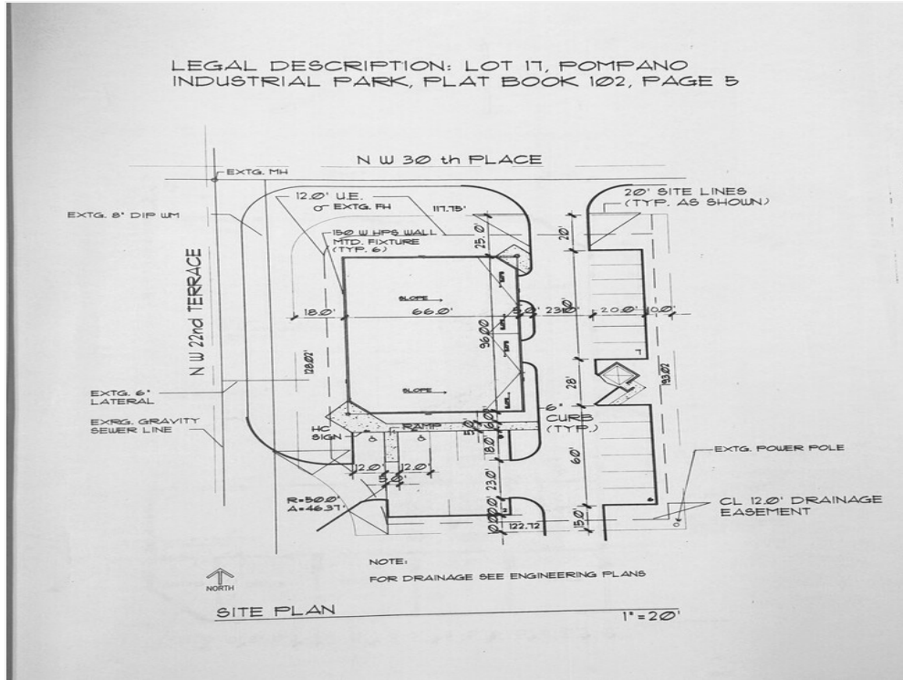
BLUEPRINT1
