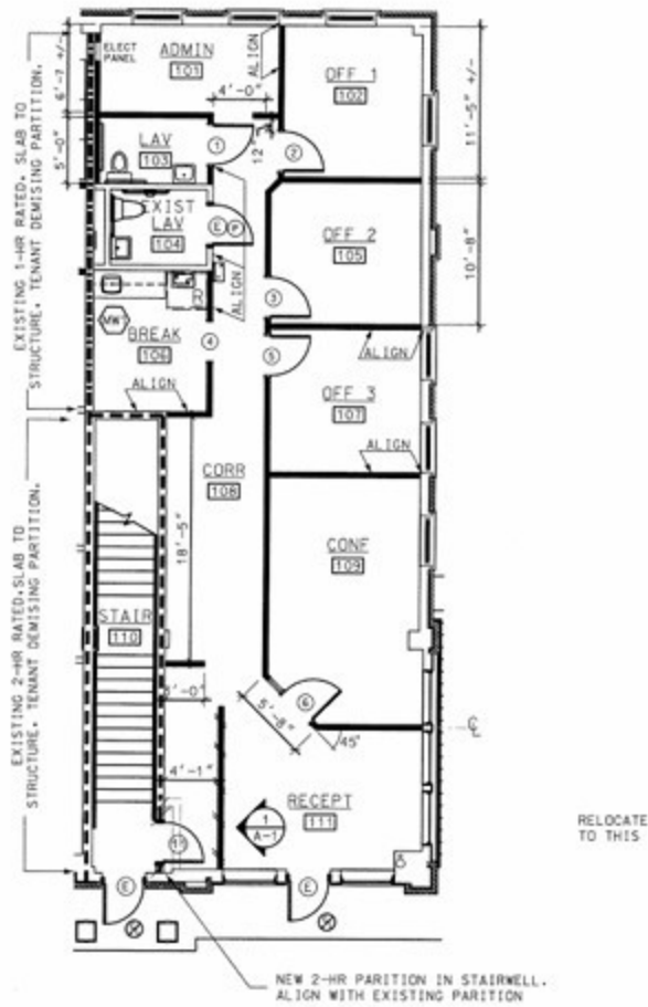
1st FLOOR ARCHITECTURAL PLAN
