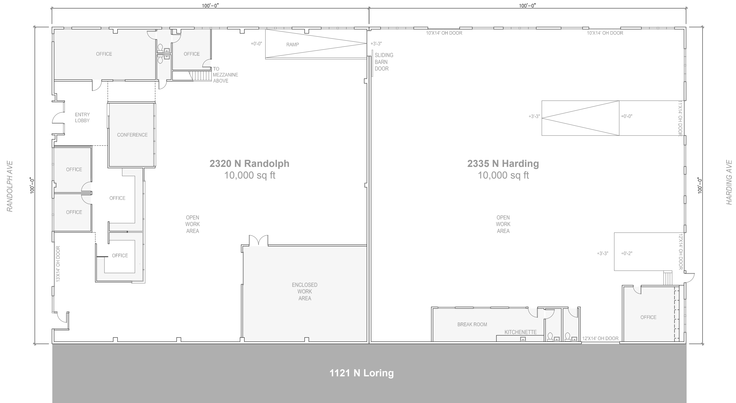
GROUND FLOOR PLAN 2320 N Randolph / 2335 N Harding
