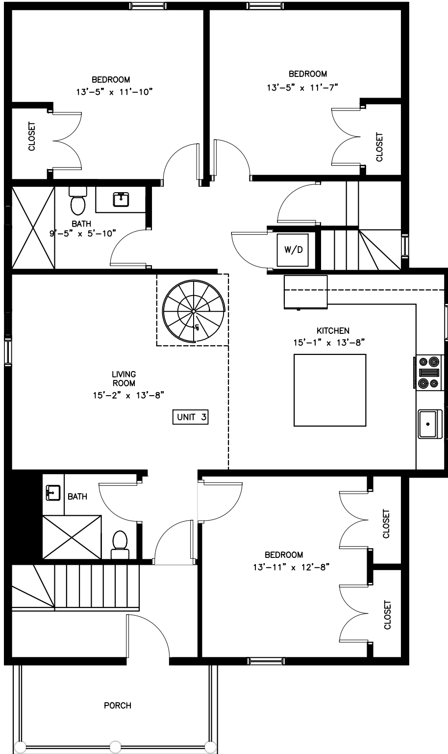
THIRD FLOOR PLAN UNIT 3
