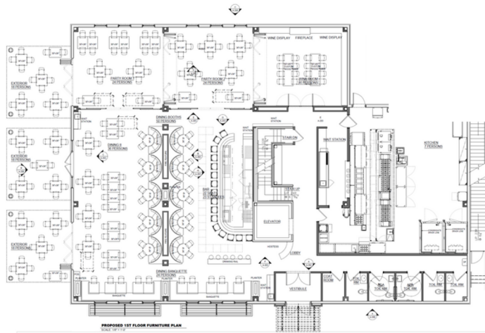
First Floor Proposal
