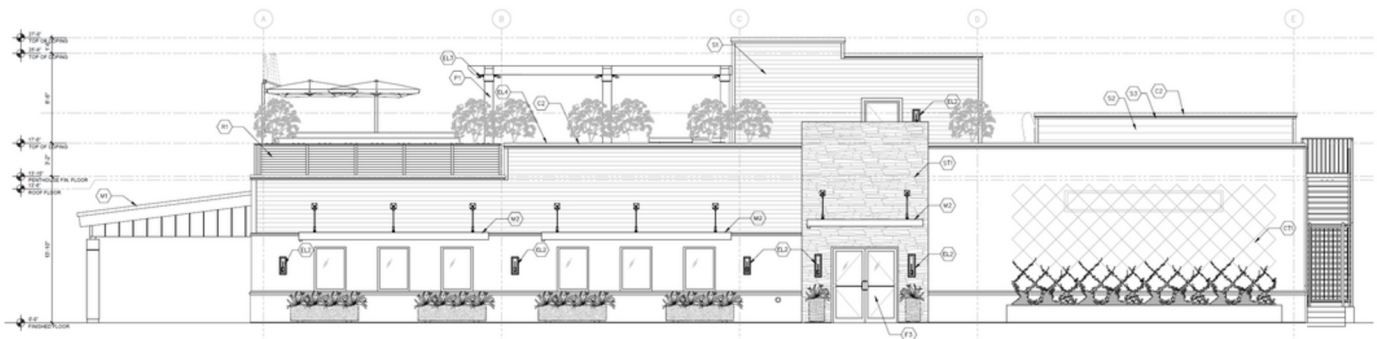
North Exterior Elevation Proposal
