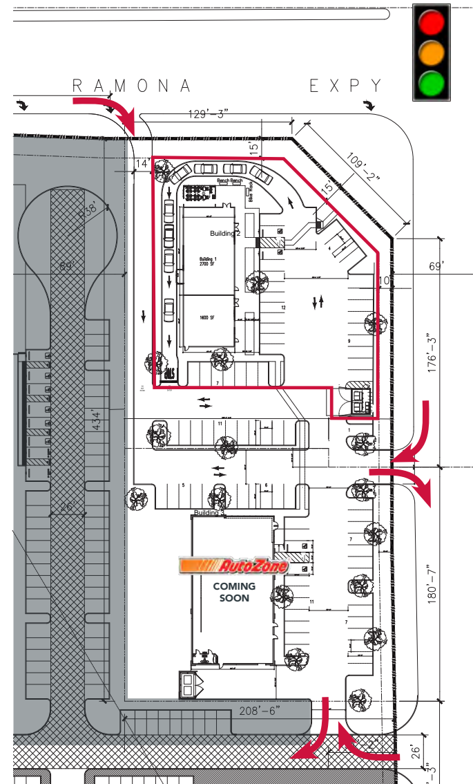
CONCEPTUAL MULTI-TENANT DRIVE THRU LAYOUT
