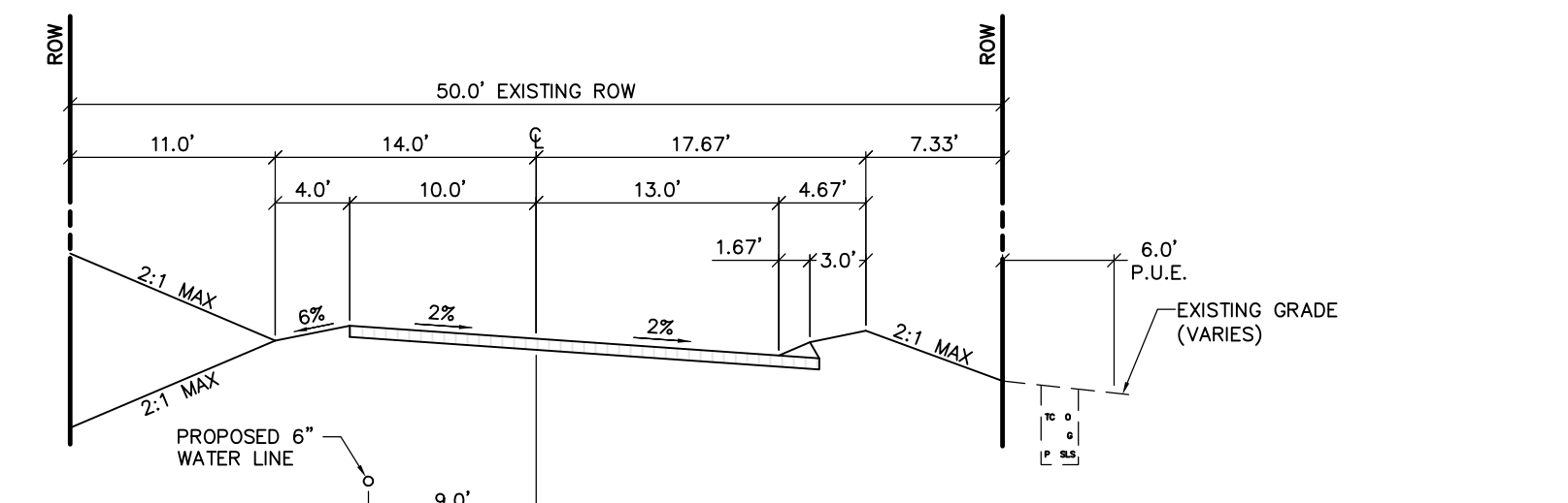
PROPOSED STAGECOACH ROAD SECTION, TYP HORIZONTAL SCALE: 1" = 10' VERTICAL SCALE: 1" = 2'
