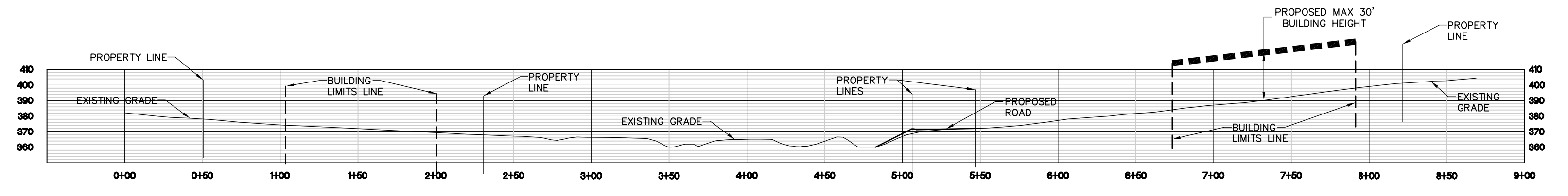
SITE CROSS SECTION HORIZONTAL SCALE: 1" = 60' VERTICAL SCALE: 1" = 60'
