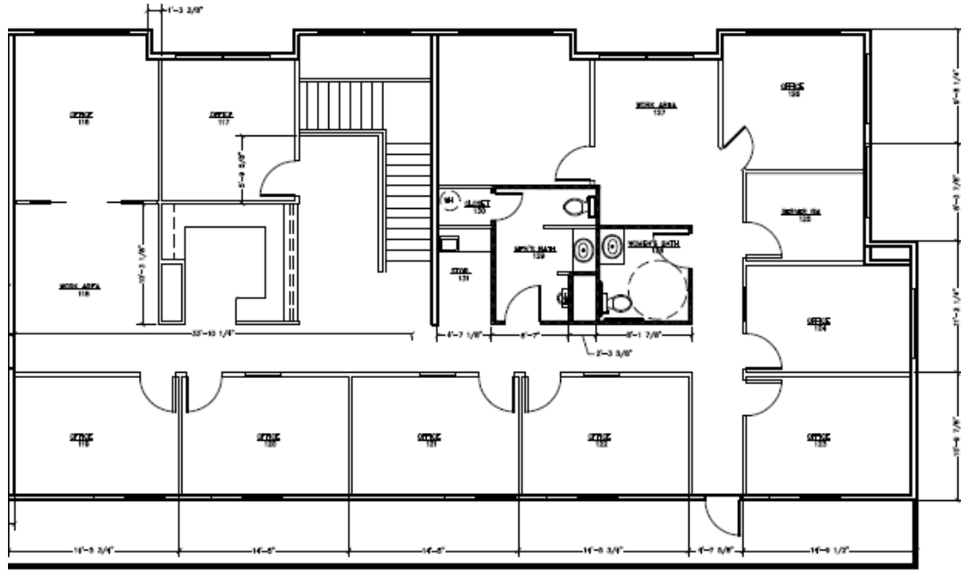
2ND FLOOR PLAN SCALE: 1/4"=1'-0"
