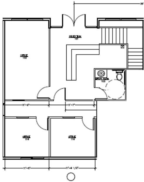
1ST FLOOR PLAN SCALE: 1/4"=1'-0"
